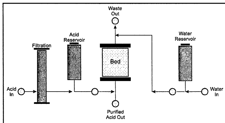
Figure 2-4. Nitric Acid Recycling
