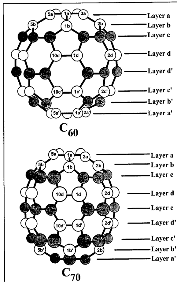
FIGURE 3-4. DIAGRAM OF A FULLERENE
