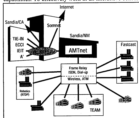
FIGURE 2-16. ADVANCED MANUFACTURING TECHNOLOGIES NETWORK
