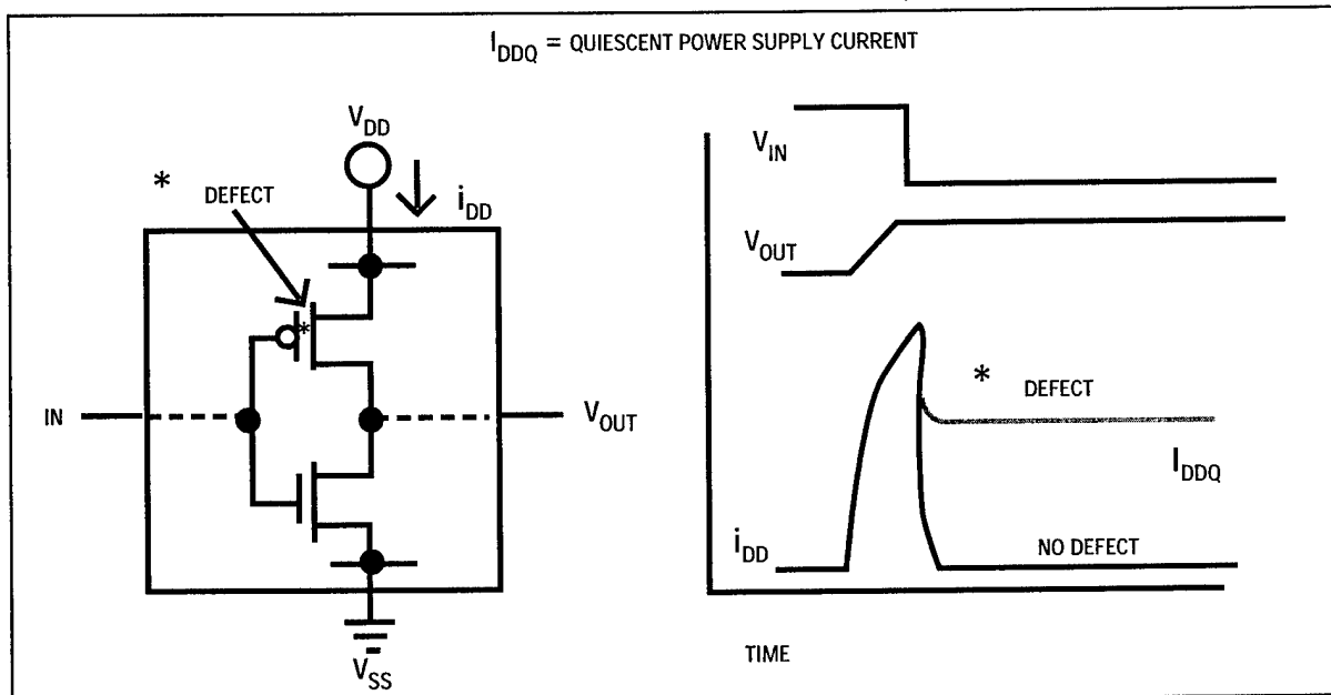
FIGURE 2-9. I_{DDQ} TESTING
