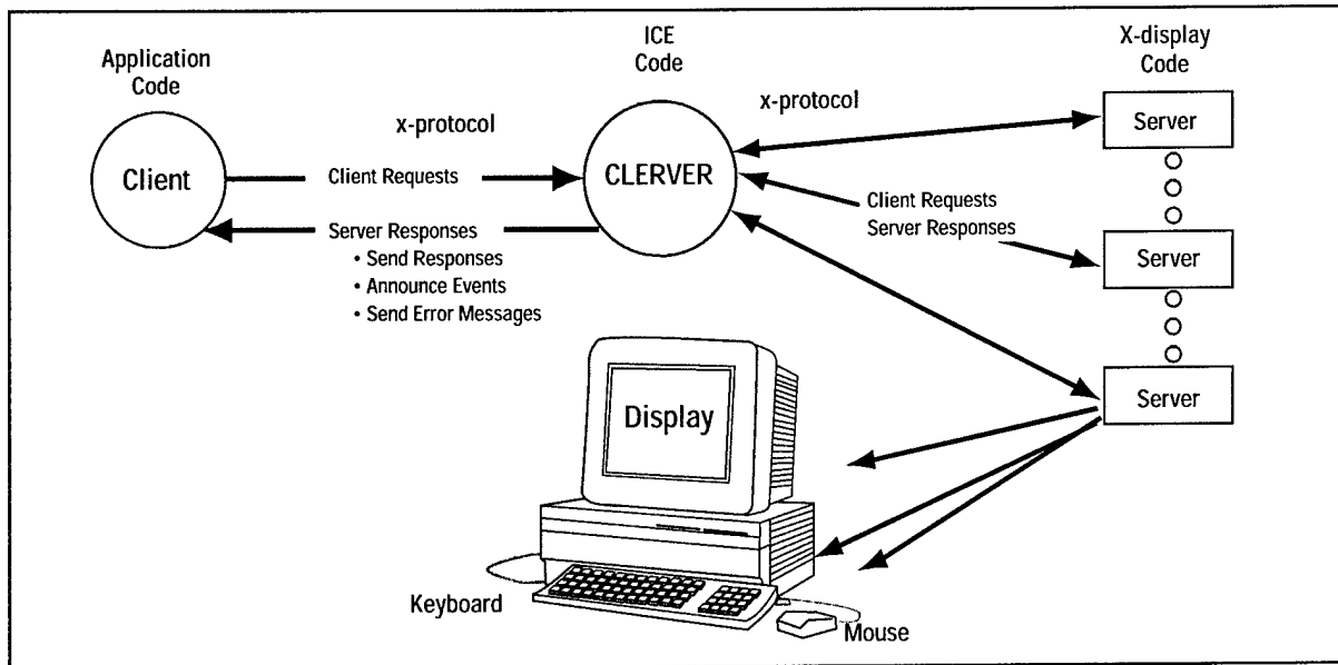
FIGURE 2-6. CLERVER SOFTWARE
