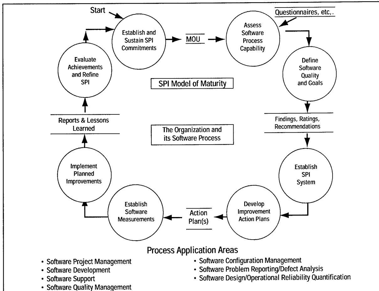
FIGURE 3-3. SOFTWARE PROCESS IMPROVEMENT METHOD
