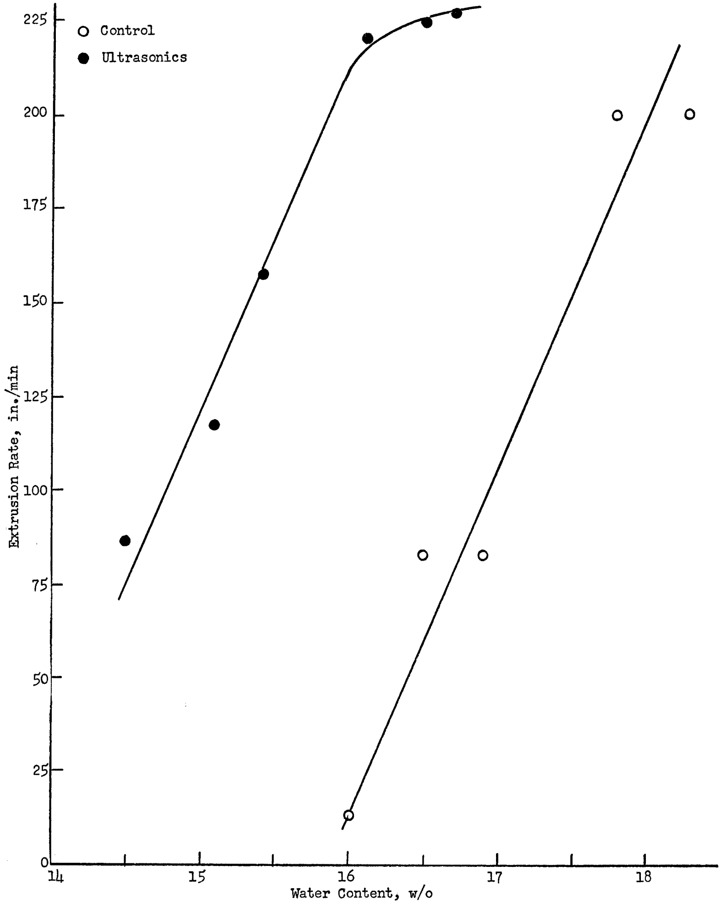
Fig. 13: RELATIONSHIP OF WATER CONTENT TO EXTRUSION RATE IN EXTRUDING ALUMINA WITH AND WITHOUT ULTRASONICS
