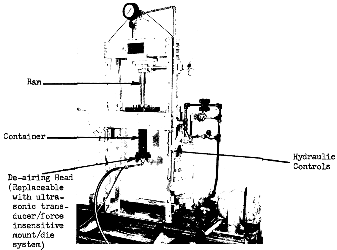
Fig. 2: HYDRAULICALLY OPERATED WILSON PRESS The de-airing flange is shown on the bottom of the holder.
