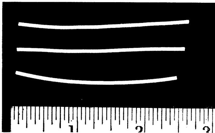
Fig. 17: SAMPLES OF 1/16-INCH TITANIA RODS EXTRUDED WITH ULTRASONIC ACTIVATION (TOP AND MIDDLE) AND WITHOUT ULTRASONIC ACTIVATION (BOTTOM)
