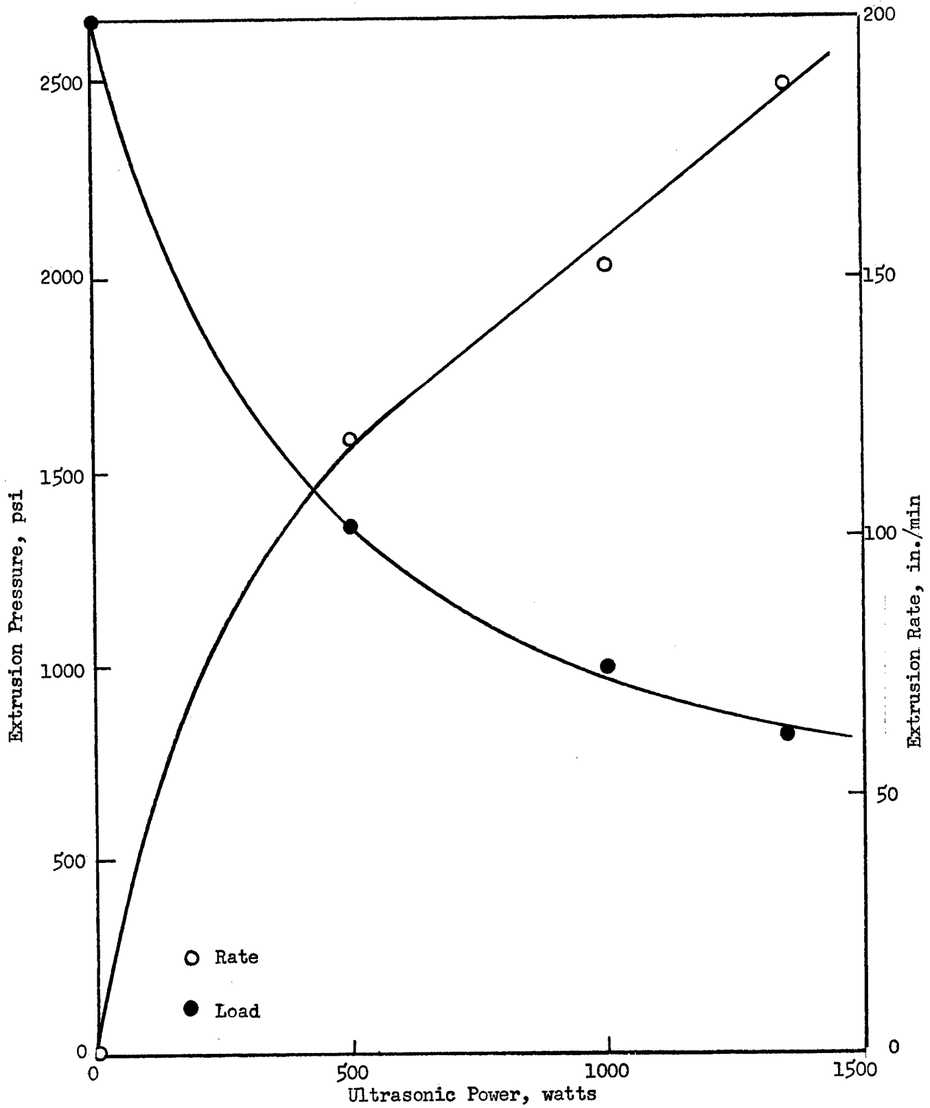
Fig. 5: RELATION OF ULTRASONIC POWER LEVEL TO EXTRUSION RATE AND PRESSURE (From Composition B, Table 1)
