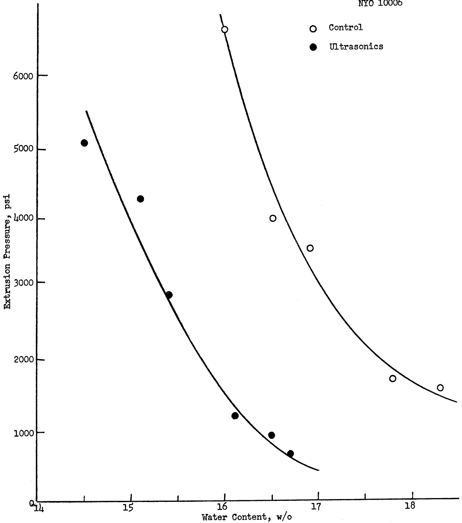
Fig. 12: RELATIONSHIP OF WATER CONTENT TO EXTRUSION PRESSURE IN EXTRUDING ALUMINA WITH AND WITHOUT ULTRASONICS
