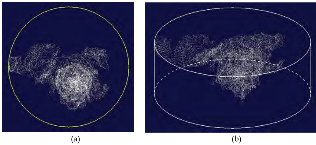
Figure 27. Combined residual penetrator point cloud of the TiB 2 disk used in test no. R-1 (2nd).
