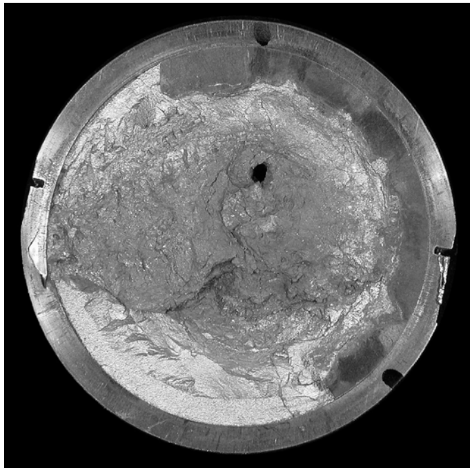
Figure 4. \text{TiB}_2 with prestress; dual impact—front surface.
