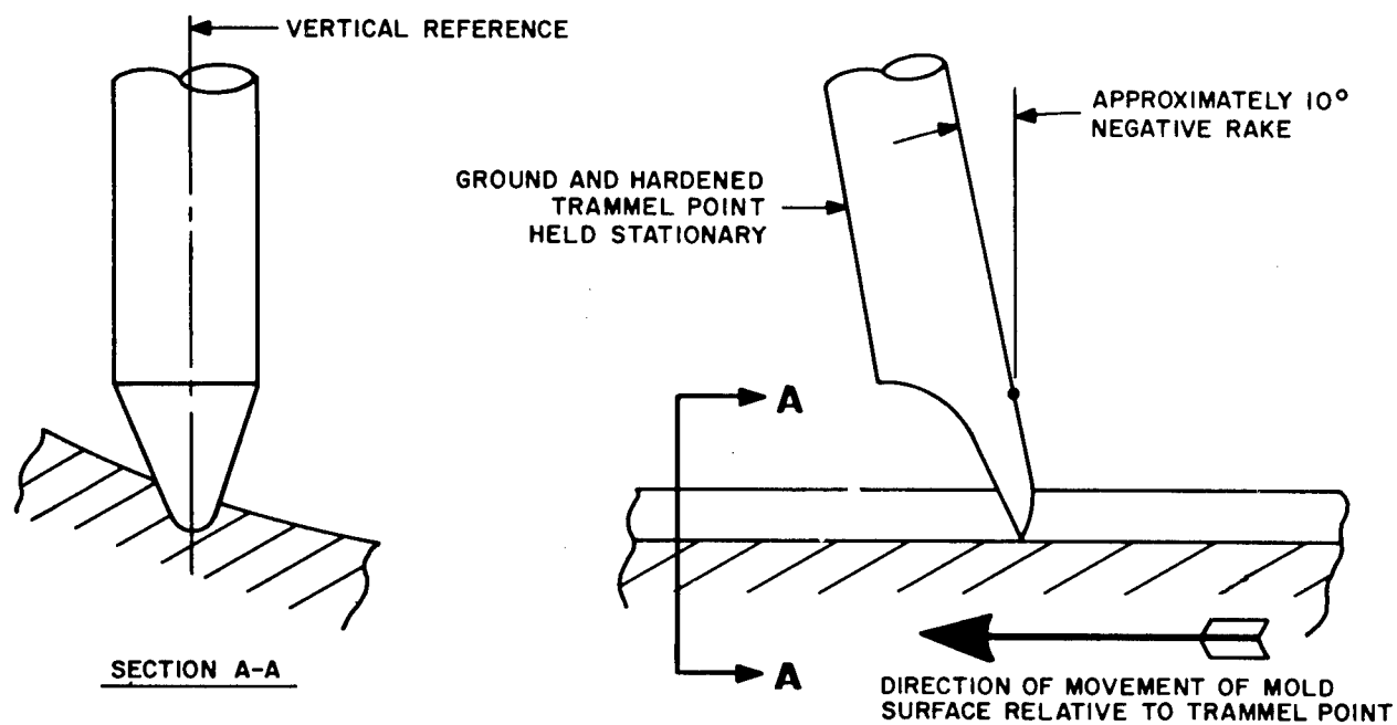
Figure D-1. Scribing of Spincast Mold
