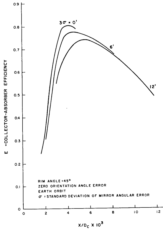
Figure 4.2-3. Collector-Absorber Efficiency
