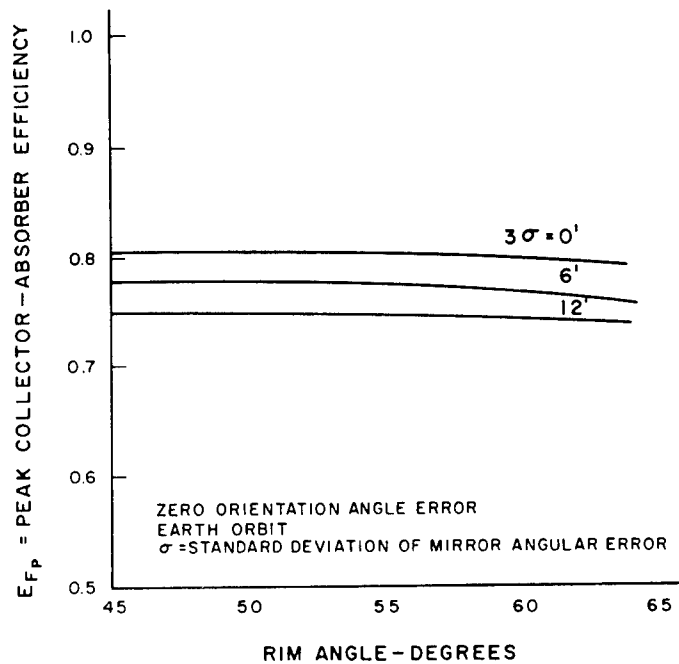
Figure 4.2-4. Peak Collector-Absorber Efficiency
