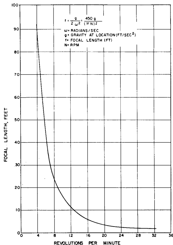
Figure 5.2-6. Focal Length vs. Spin Speed
