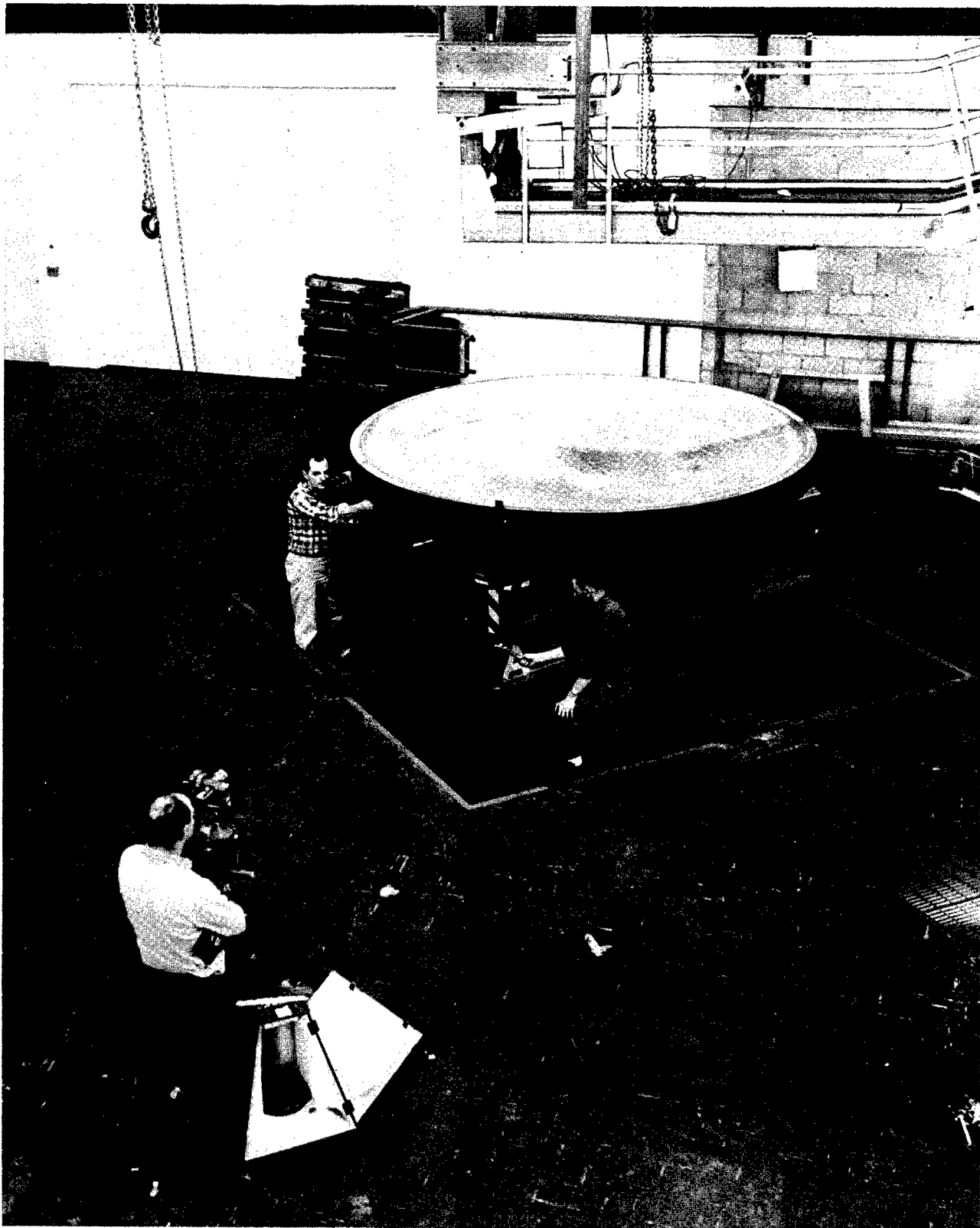
Figure 5.1-4. Spincast Mold Mounted on Spintable
