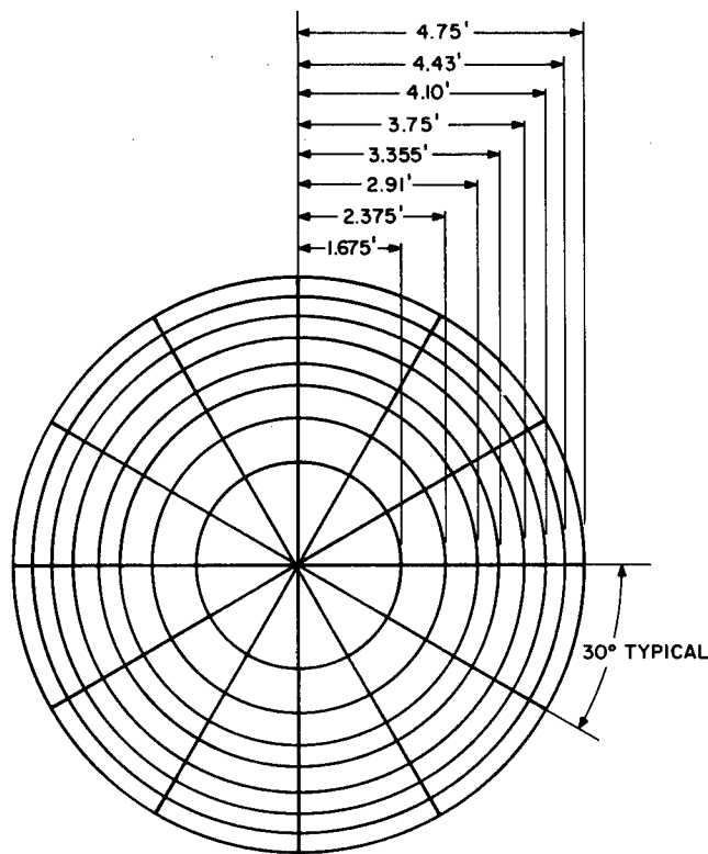
Figure 5.5-3. Subdivision of Mirror Surface Into 96 Equal Areas
