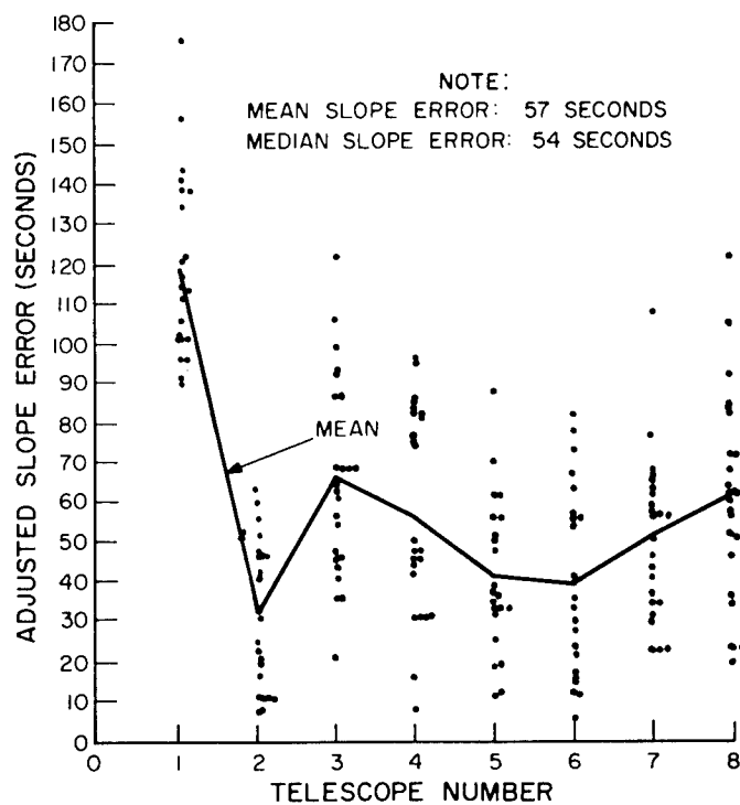
Figure 5.5-10. Optical Inspection of Final Spincast Coat; Adjusted Slope Errors
