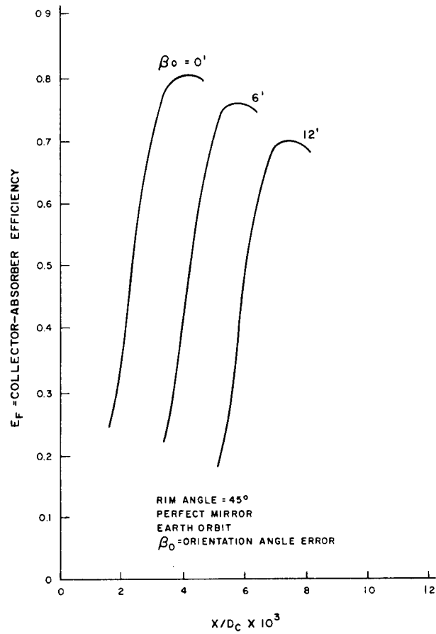
Figure 4.3-1. Collector-Absorber Efficiency
