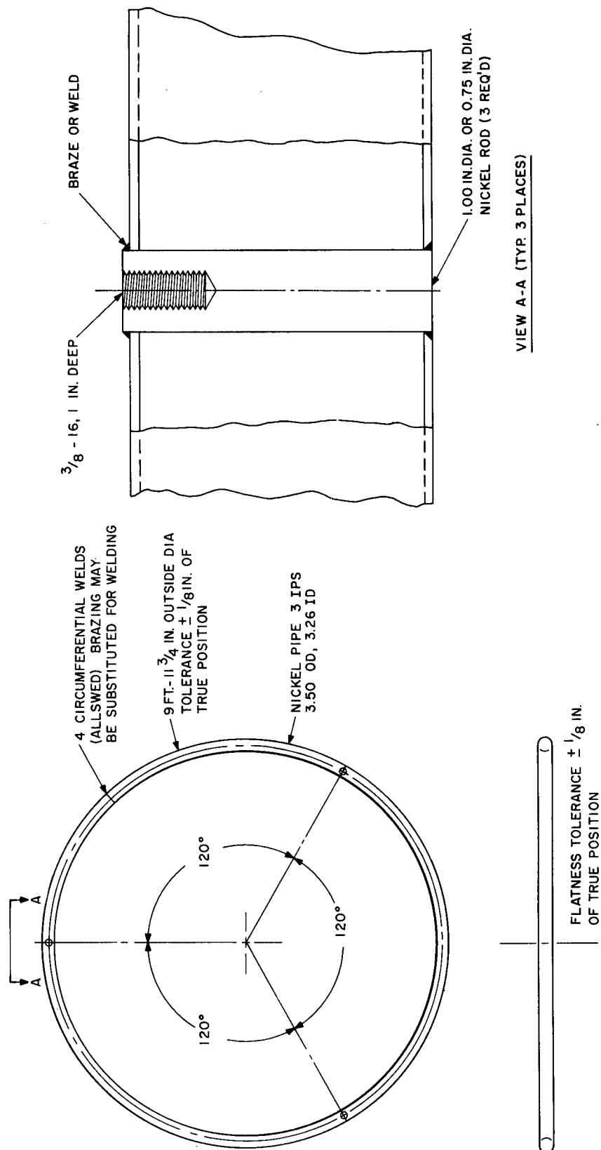
Figure 7.3-2. Mirror Support Torus
