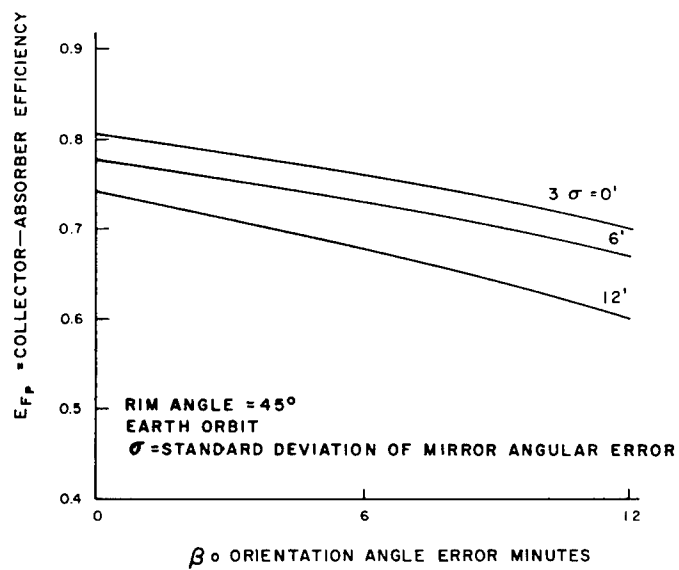
Figure 4.1-2. Peak Collector-Absorber Efficiency
