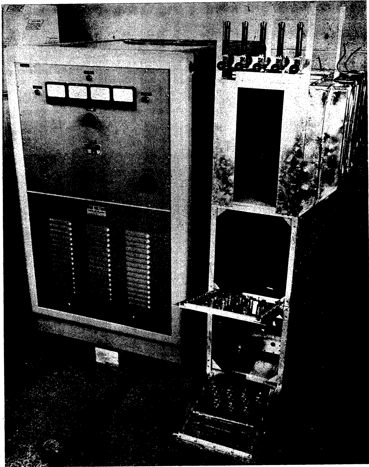
Figure 16. Arrangement for crystal growing with the R. F. plasma heat source.
