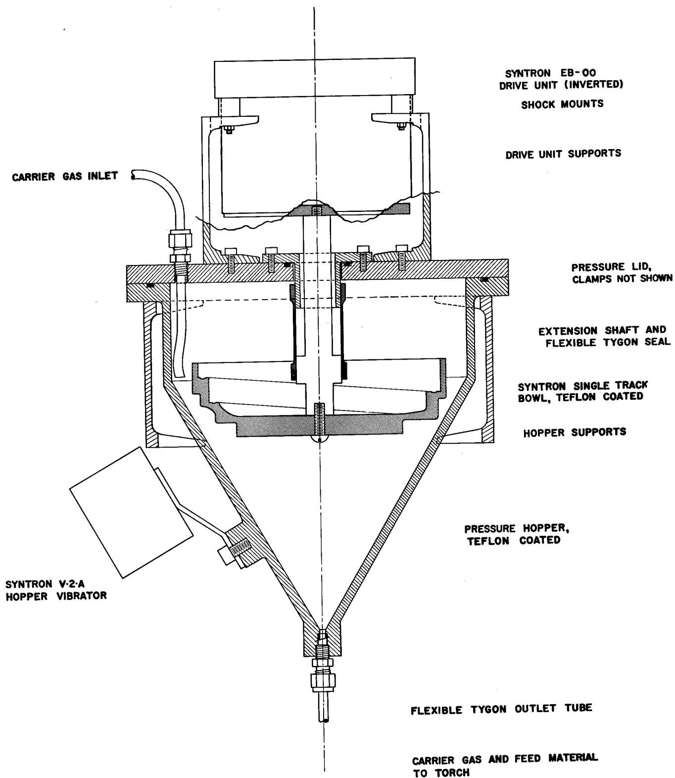
Figure 12. Pressurized material feeder for crystal growth.
