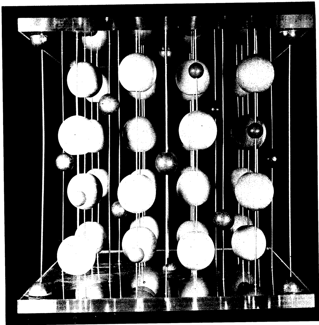
Figure 2. Model of spinel unit cell viewed along [100].
