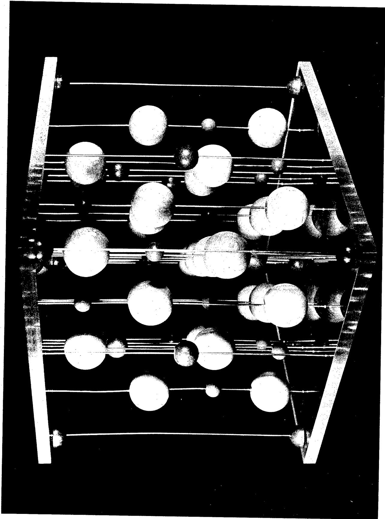
Figure 3. Model of spinel unit cell viewed along [110] .
