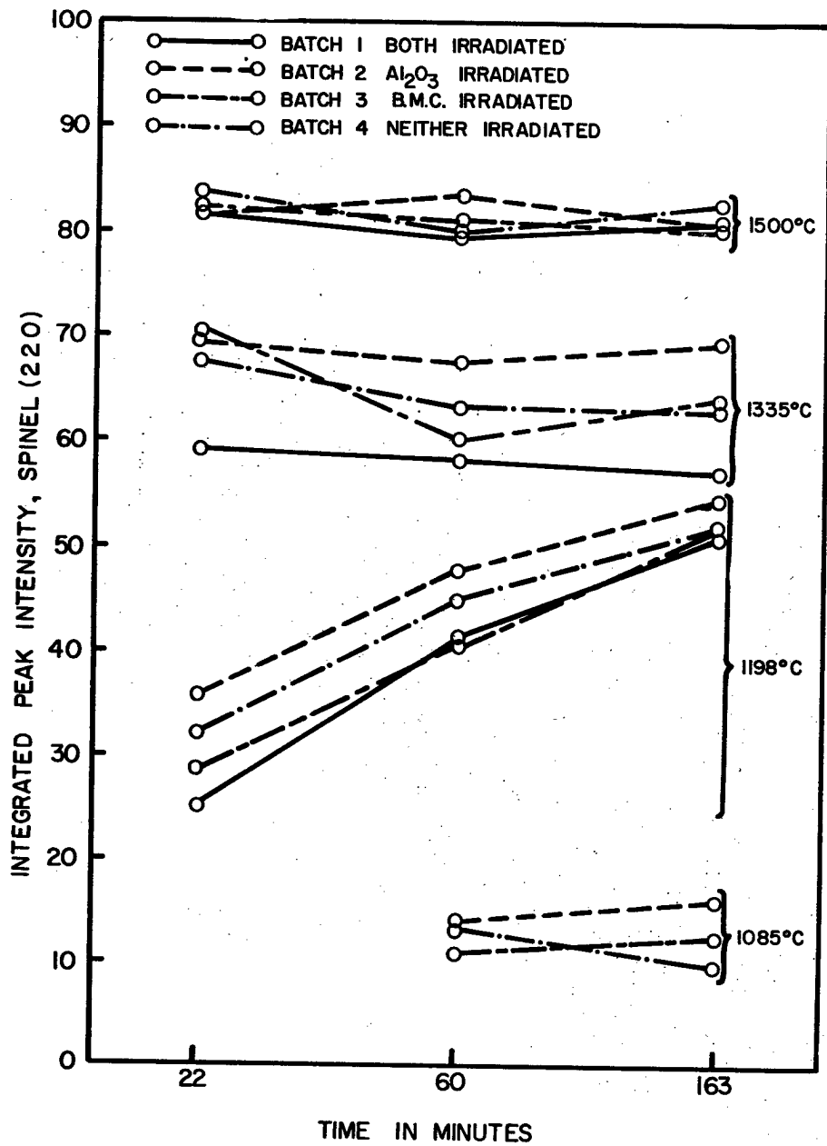
ISOTHERMAL CONVERSION TO SPINEL AS A FUNCTION OF \ln(t) FOR IRRADIATED AND UNIRRADIATED ALUMINA-BASIC MAGNESIUM CARBONATE MIXTURES.
