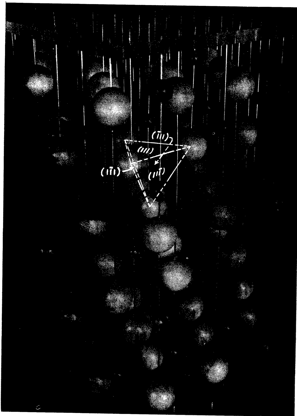
Figure 5. Spinel crystal model showing intersections of {111} planes.
