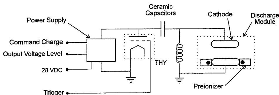
Figure 3-4. Pulsed power system.
