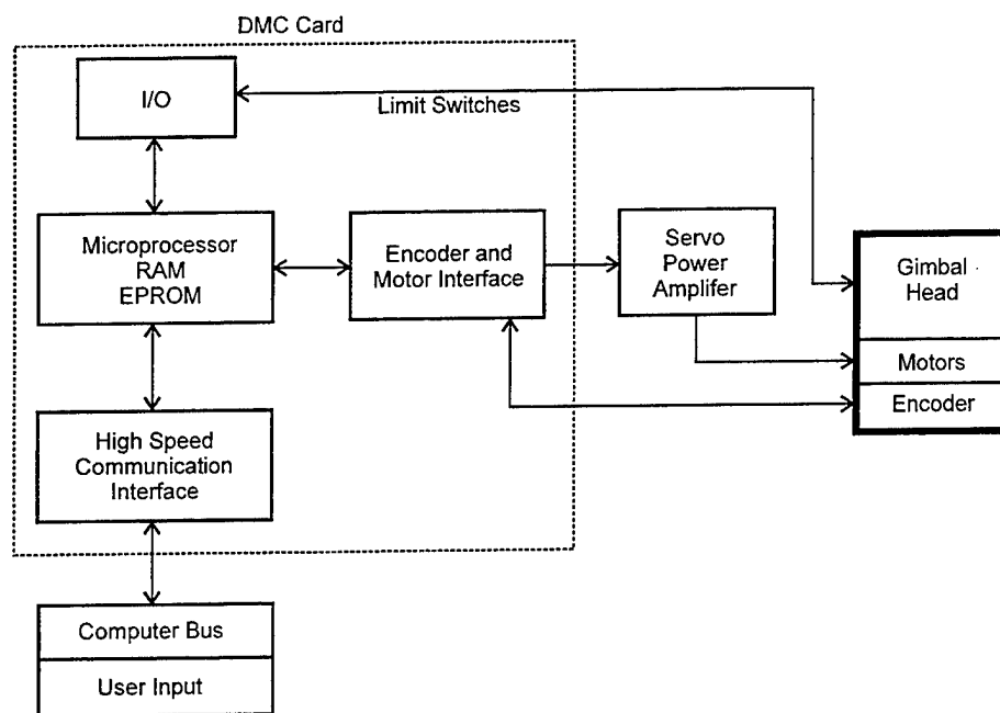
Figure 4-4. Gimbal functional block diagram.
