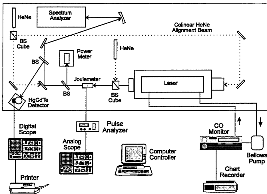
Figure 3-38. Qualification test diagnostic setup.
