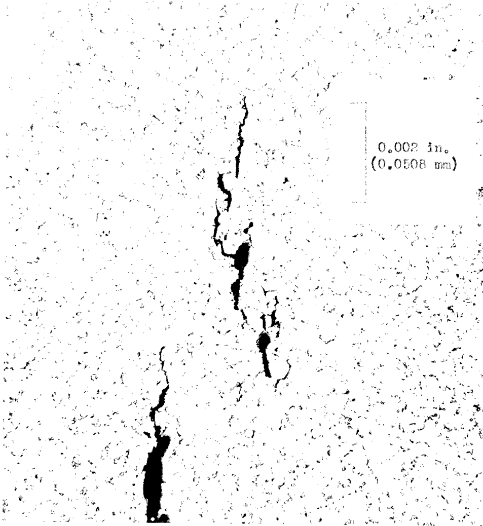
Figure 9.- Photomicrograph of specimen 54 showing length and discontinuous nature of cracks in residually stressed, salt-dipped Ti-8Al-1Mo-1V exposed at 550° F (561° K) for 507 hours. L-65-7
