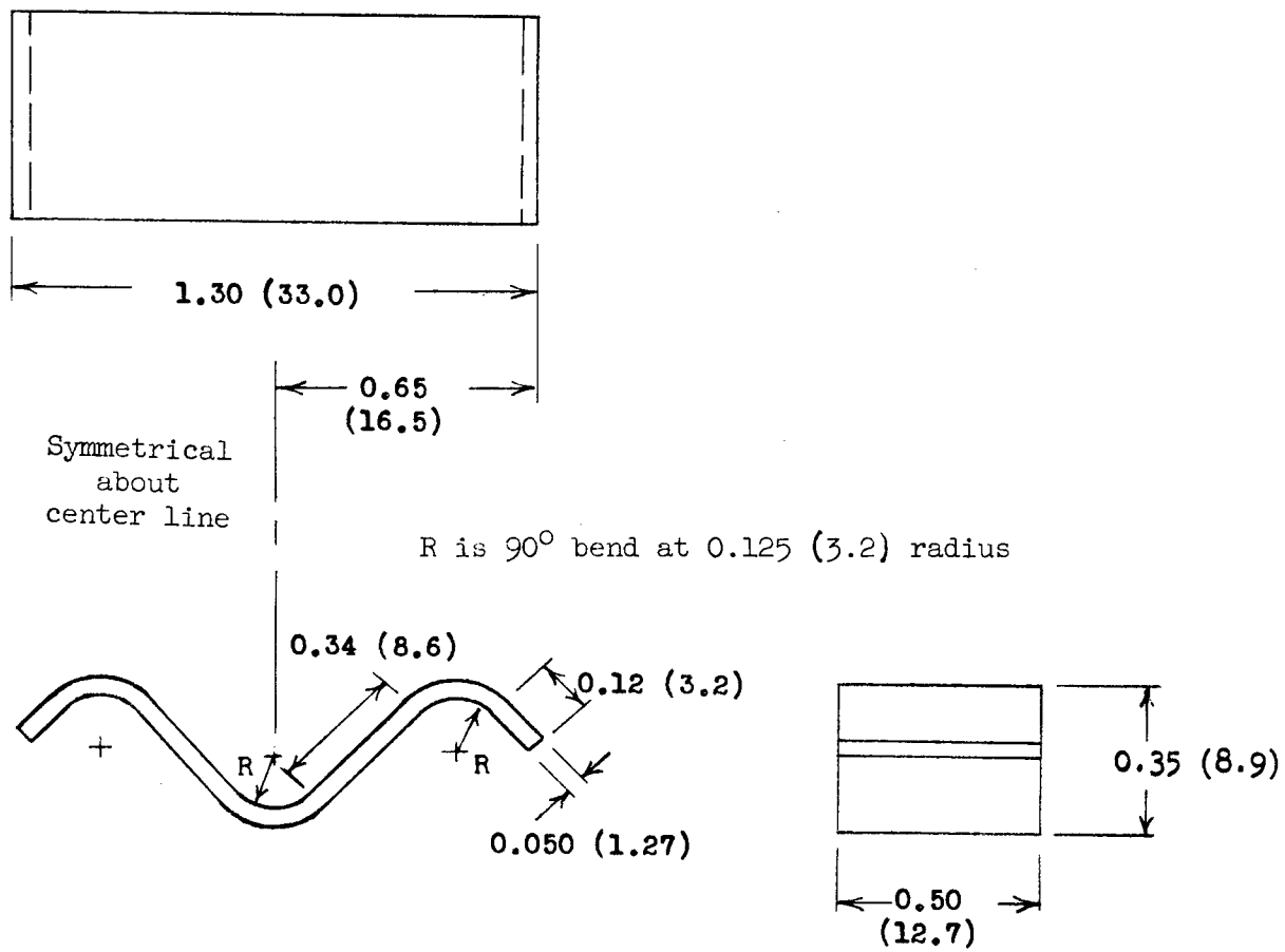
Figure 1.- Residually stressed specimen design. Principal dimensions are in inches; dimensions in parentheses are in millimeters.
