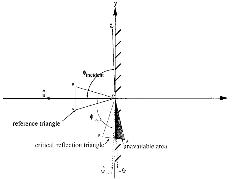
Figure 2: Critical reflection triangle. Shaded triangle is a nonactive area.
