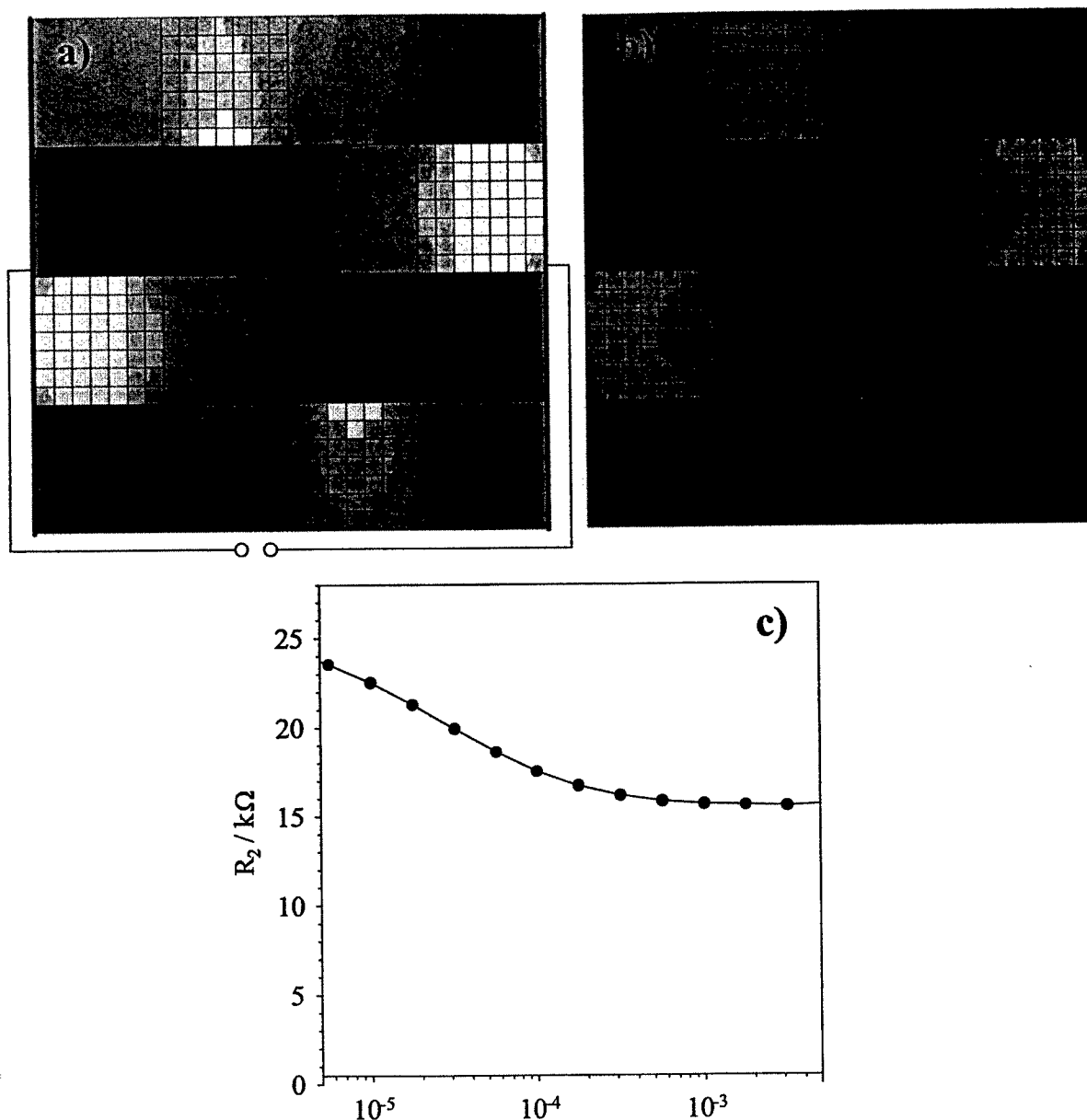
Fig. 3. Top: magnitude of the d.c. current density within the two-dimensional polycrystal of Fig. 2 for two different bulk conductivities: (a) \sigma_{\text{bulk}} = 2 \times 10^{-4} 1/\Omega ; (b) \sigma_{\text{bulk}} = 10^{-5} 1/\Omega . For other parameters see Fig. 2. Dark indicates high current density and light low current density. Bottom: resistance from the low-frequency semicircle R_2 as a function of bulk conductivity.
