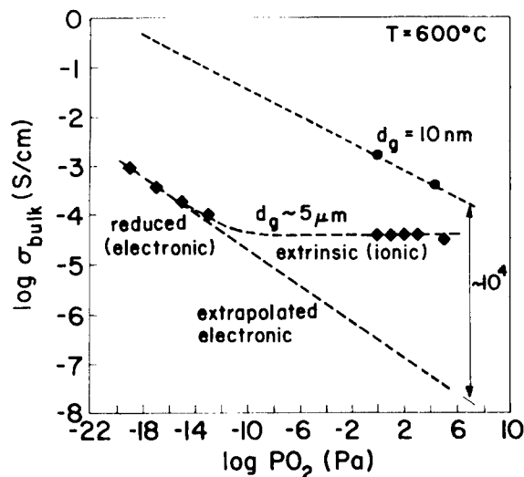
Fig. 11. The bulk conductivity of nanocrystalline ( d \sim 10 nm) and coarsened microcrystalline ( d \sim 5 \mu\text{m} ) \text{CeO}_{2-x} measured at 600°C as a function of oxygen partial pressure [11].
