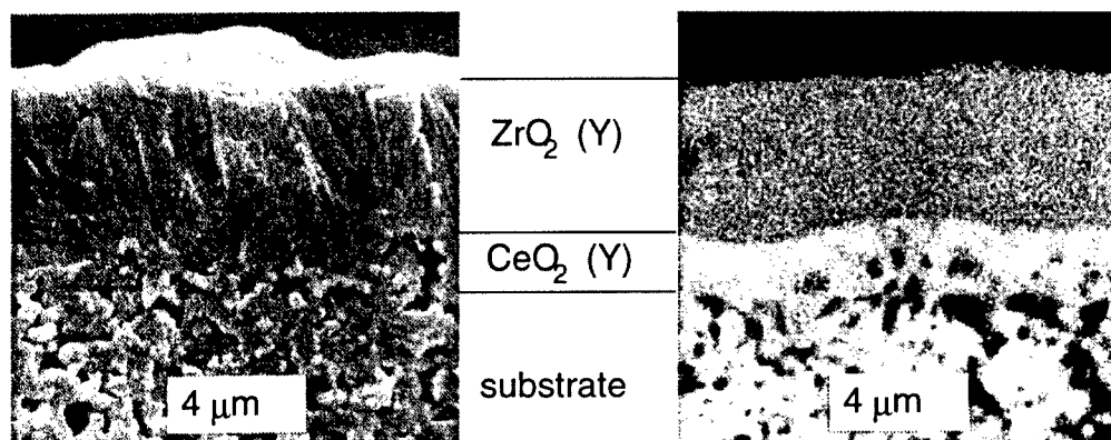
Fig. 8. SEM picture (left) and elemental analysis (right) of an electrolyte bilayer deposited via DC sputtering on top of a porous cathode substrate. It consists of a 1- \mu\text{m} thick \text{CeO}_2 (Y) chemical compatibility layer and a 4- \mu\text{m} thick \text{ZrO}_2 (Y) electrolyte layer [94].
