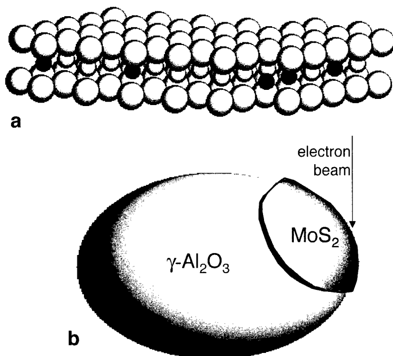
Fig. 7. Schematic representation of the morphology of MoS 2 particles and their location on the \gamma\text{-Al}_2\text{O}_3 substrate. The position of the Co atoms at the edges is illustrated in (a). The dark small atoms are Co atoms, and the large and small bright atoms are S and Mo, respectively. The covering of the \gamma\text{-Al}_2\text{O}_3 particle by the MoS 2 particle like a blanket is illustrated in (b).
