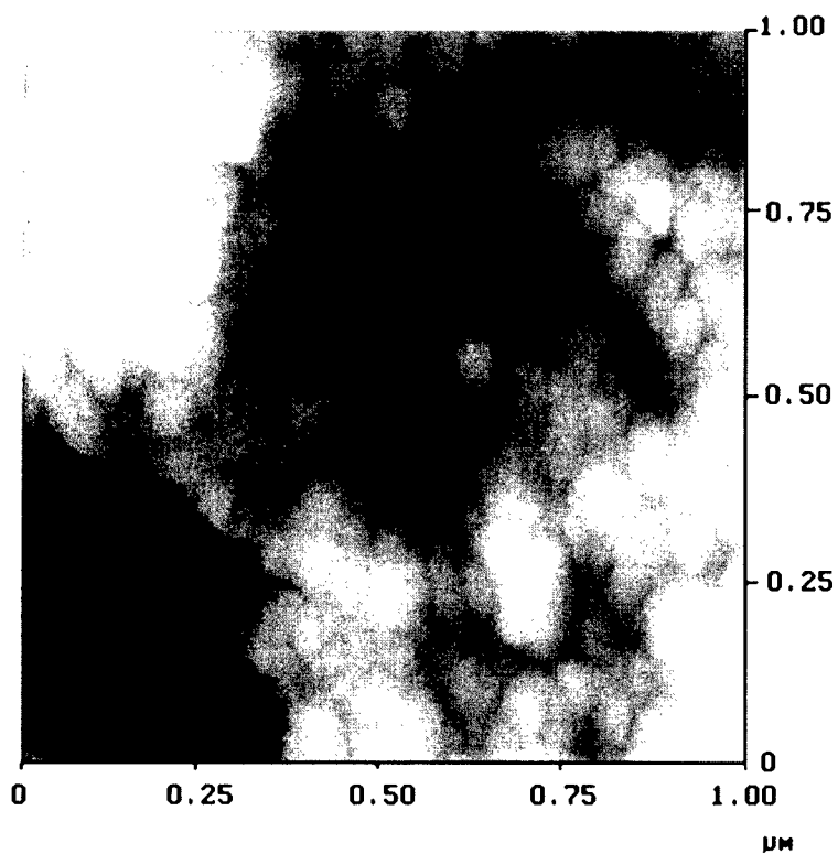
Fig. 7. Contact AFM image of the surface of an electrodeposited \delta - \text{Bi}_2\text{O}_3 film grown on a (111) textured Au EQCM electrode. The scan size is 1.0\ \mu\text{m} in both directions. The average particle size is 65 \pm 6\ \text{nm} .
