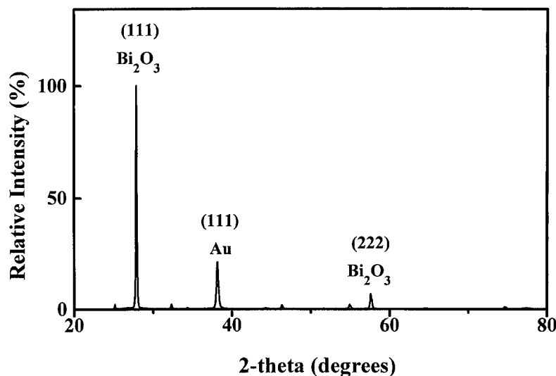
Fig. 5. XRD pattern of a \delta\text{-Bi}_2\text{O}_3 deposited onto a (111)-textured Au EQCM electrode. Comparison of this pattern with that shown in Fig. 1 reveals that the \delta\text{-Bi}_2\text{O}_3 has a strong (111) preferred orientation, suggestive of an epitaxial relationship between Au and \delta\text{-Bi}_2\text{O}_3 .
