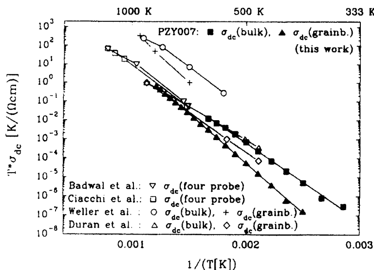
Fig. 7. Comparison of bulk and grain boundary conductivities of nano- and micro-crystalline YSZ [14].
