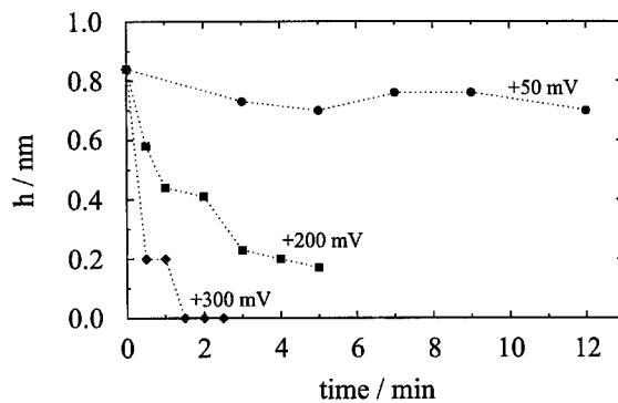
Fig. 7. Variation of cluster height with time during the dissolution of Ag clusters on Au(111) at various electrode potentials.
