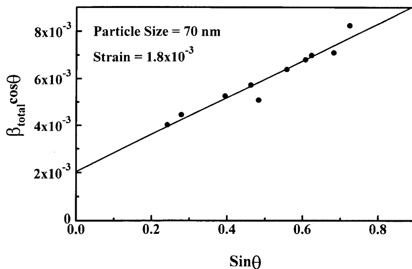
Fig. 2. Williamson-Hall plot for \delta\text{-Bi}_2\text{O}_3 from X-ray powder pattern. A particle size of 70 nm was obtained from the y-intercept of the plot, while the strain ( \Delta d/d ) was determined from the slope of the line to be 1.8 \times 10^{-3} . Linear regression gave a correlation coefficient of 0.97.
