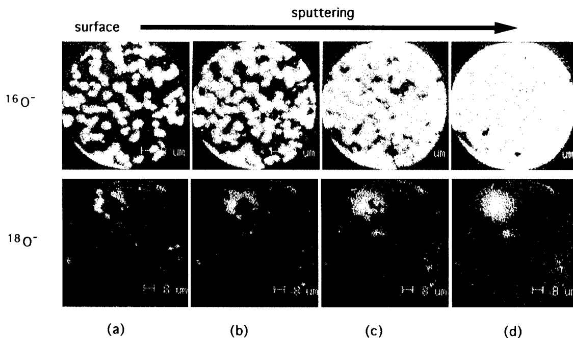
Fig. 11. ^{16}\text{O}^- and ^{18}\text{O}^- distribution in the sample treated at 773 K in 0.2 bar oxygen ^{18}\text{O} under cathodic polarization ( -0.5\text{ V} ) for 5 min. Images were taken at the surface (a); after sputtering 2 min. (b); 4 min. (c); and 6 min. (d).
