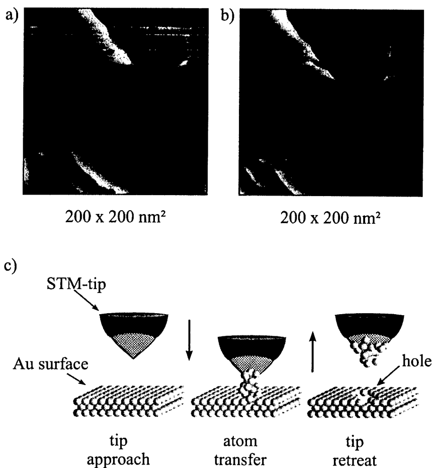
Fig. 8. (a) STM image of a Au(111) electrode in 1 mM \text{NiSO}_4 + 10 mM \text{H}_3\text{BO}_3 + 0.2 mM \text{HCl} , showing the hole formation with a Ni-covered Pt–Ir tip. The five lines in the upper part of the image reflect the pulses on the z-piezo (five pulses per line). E_{\text{sample}} = -320 mV vs. SCE, E_{\text{tip}} = -470 mV, I_t = 2 nA. (b) Same area, imaged 1 min later. E_{\text{sample}} = -320 mV vs. SCE, E_{\text{tip}} = -470 mV, I_t = 2 nA. (c) Suggested mechanism of the hole formation in the Au(111) substrate during the approach of a Ni-covered STM tip.
