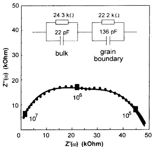
Fig. 10. Complex impedance spectrum of nanocrystalline \text{CeO}_{2-x} at 130°C in a hydrogen atmosphere and equivalent circuit [21]. Note strong overlap of high and low frequency semicircles.
