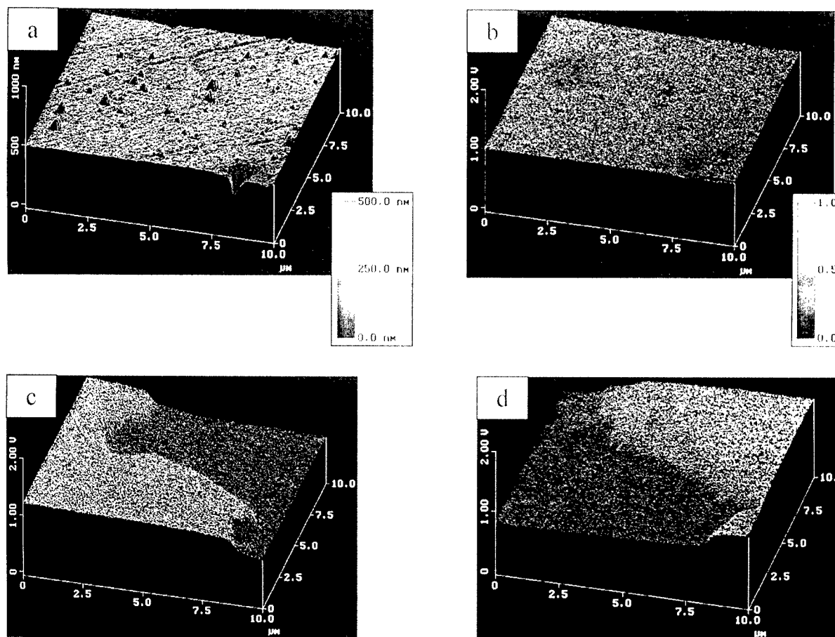
Fig. 6. Topographic structure (a) and surface potential of unbiased region of a polycrystalline ZnO surface. Surface potential variation at a grain boundary with laterally applied (c) forward and (d) reverse bias ( \pm 1.00 V applied approximately 30\ \mu\text{m} to the left and right).
