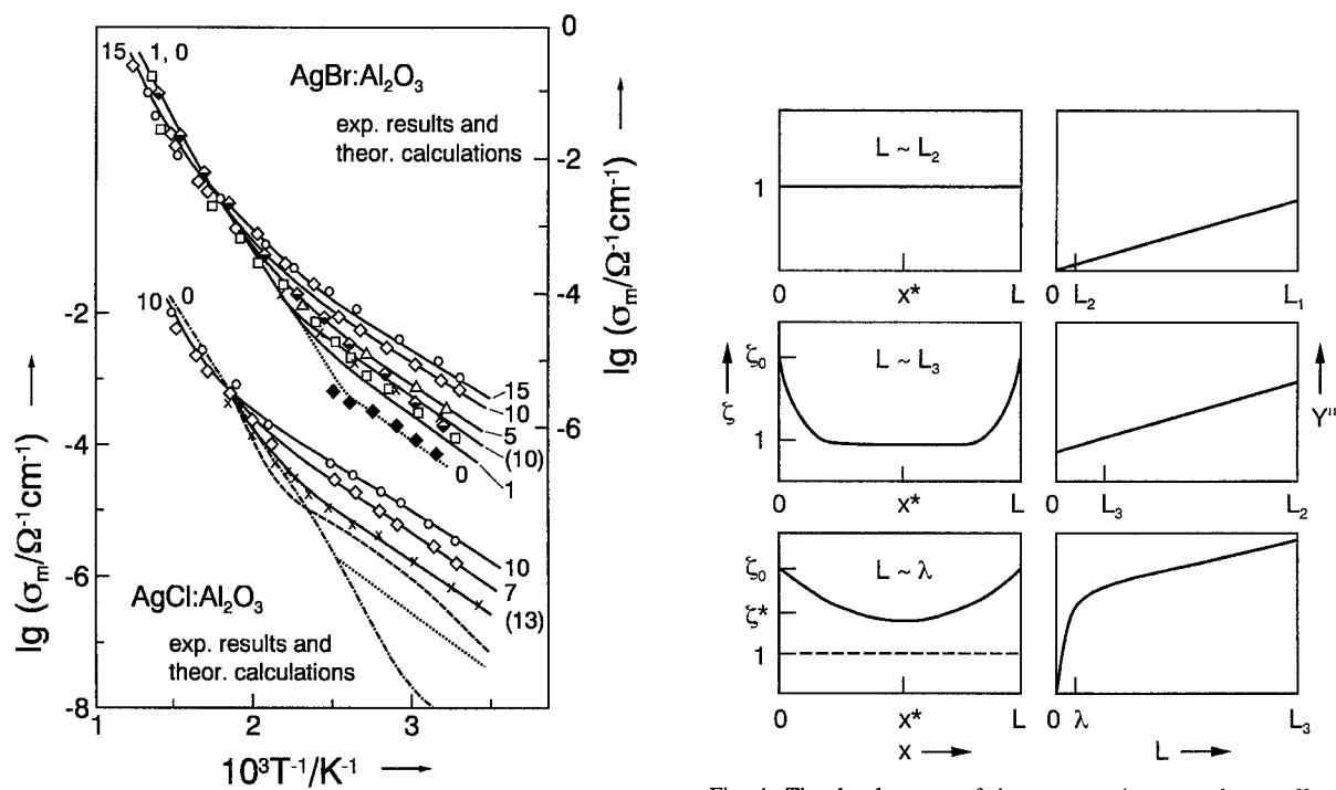
Fig. 3. The effect of 'heterogeneous doping' of AgCl and AgBr can be quantitatively interpreted by space charge effects [25].
