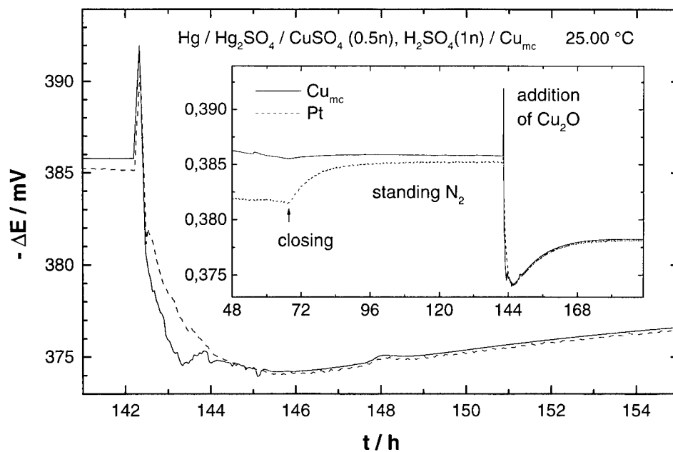
Fig. 6. Potentiometric study of the dissolution of 0.4 mg Cu_2O in 45 ml of the solution.
