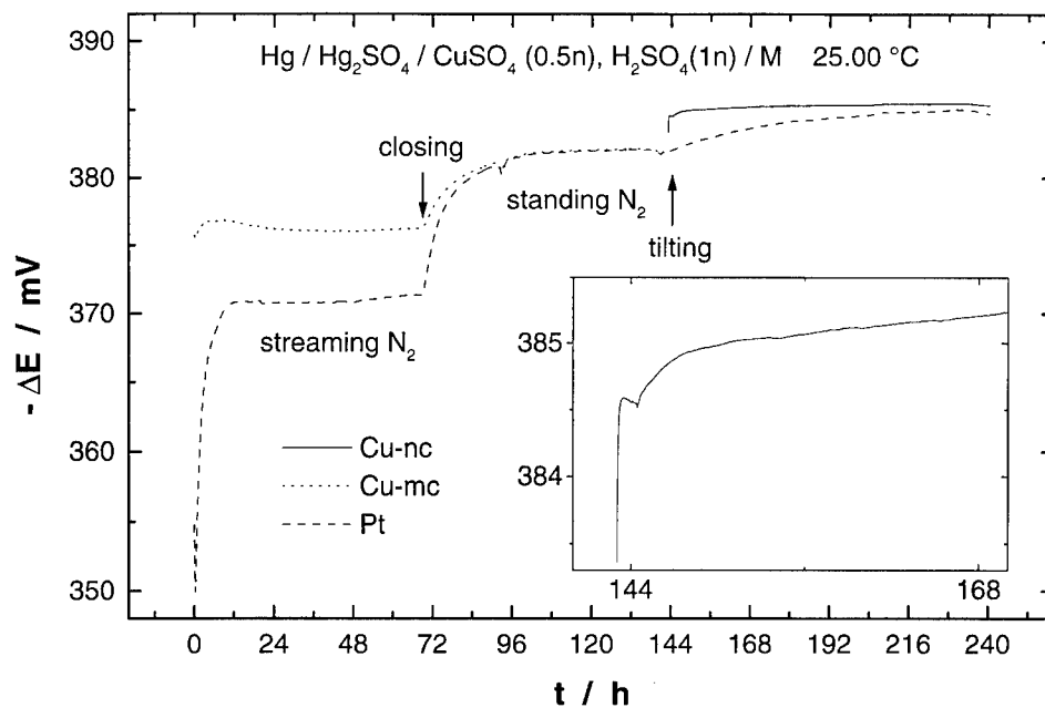
Fig. 5. Electrodes of Pt, micro- and nanocrystalline ( r=45 nm) copper in a tiltable cell. N_2 contains 40 ppm O_2 ; in the closed cell O_2 is trapped by Cu_{mc} ; by tilting Cu_{mc} is pulled out and Cu_{nc} dipped into the solution.
