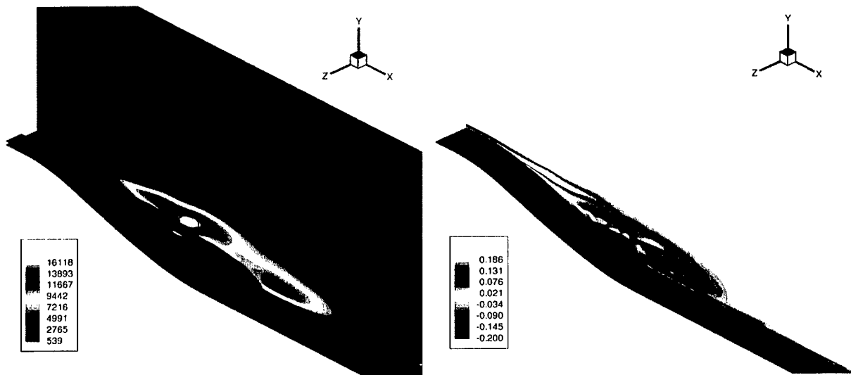
Figure 6.28: 3-D FSM computation. Instantaneous data. Left: Isosurfaces of \omega_z = -0.05, 0.05 (red, blue), and isocontours of \mu_T/\mu . Right: Isosurfaces of \omega_x = -0.02, 0.02 (red, blue), and isocontours of \omega_z .
