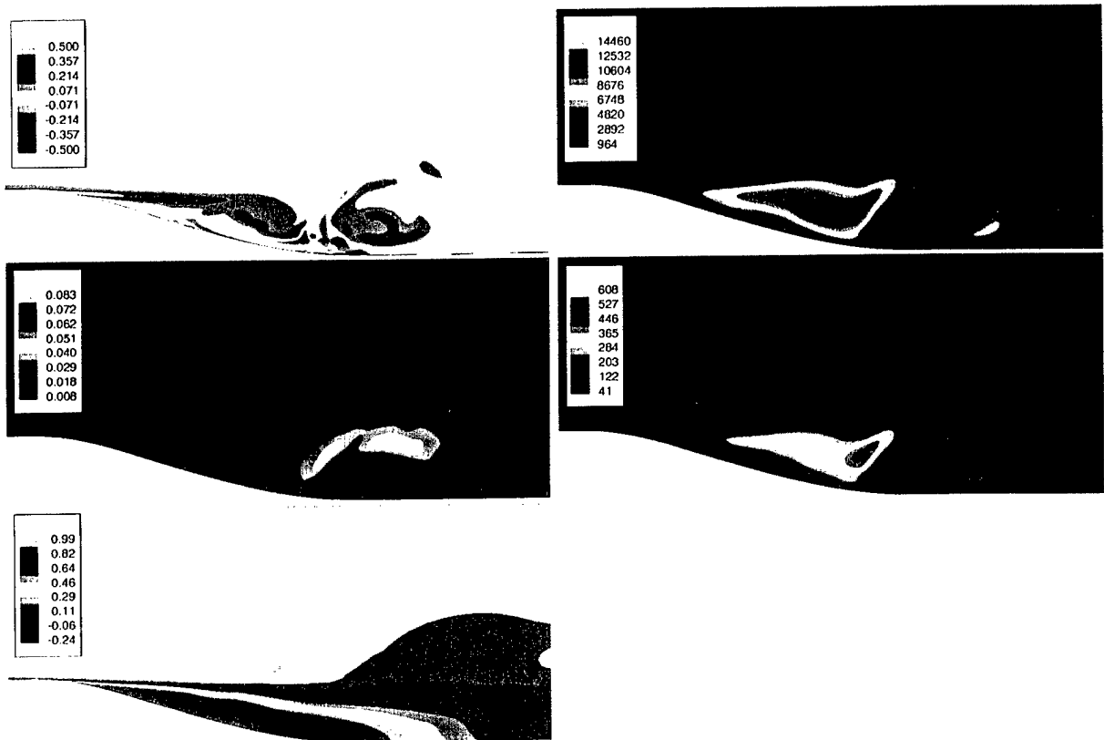
Figure 6.26: 3-D FSM computation. Slices at constant z = 0 . Top: \omega_z isocontours and \mu_T/\mu isocontours. Center: f isocontours and f\mu_T/\mu isocontours. Bottom: u isocontours (time-averaged).
