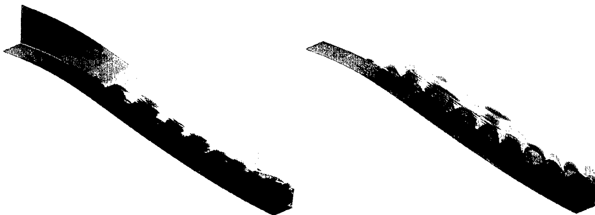
Figure 2.8: POD of 3-D DNS, mode 2. Isosurfaces of u = -0.005, 0.005 (red, blue) and isocontours of u (left). Isosurfaces of v = -0.003, 0.003 (red, blue), and isocontours of v (right).
