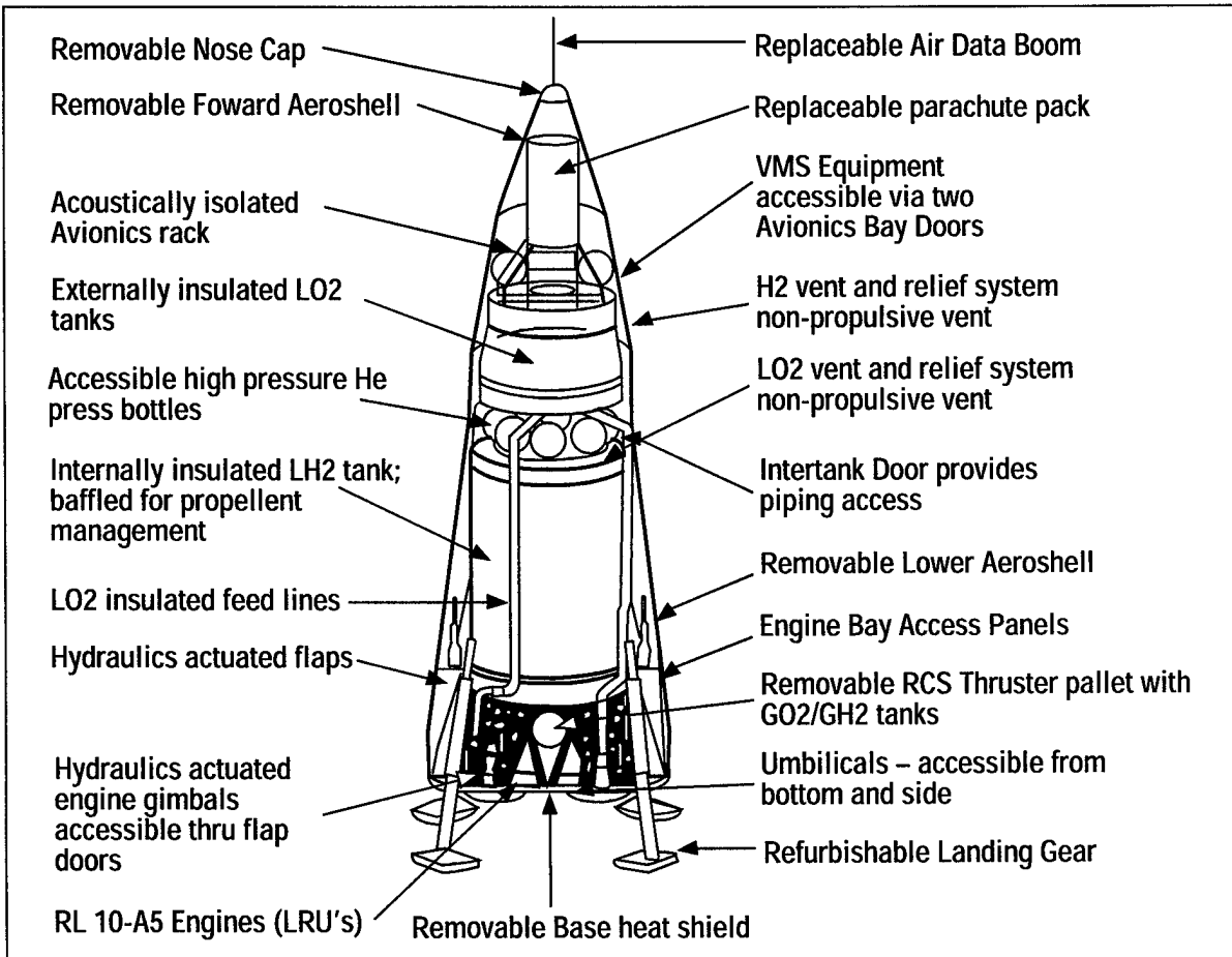
FIGURE 3-8. DC-X VEHICLE
