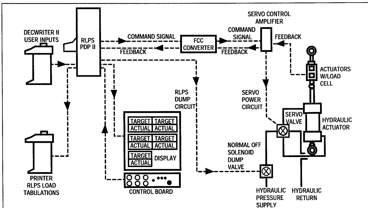
FIGURE 3-7. AUTOMATED LOAD PROGRAMMING SYSTEM
