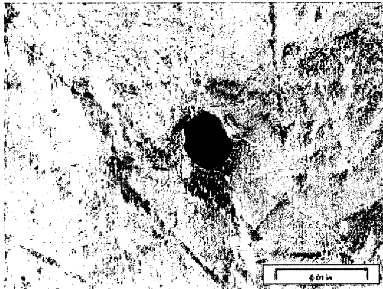
Figure 15. Microporosity Within the Narrow Gap Magnetically Impelled Weldment (Etchant: Kroll's Reagent).
