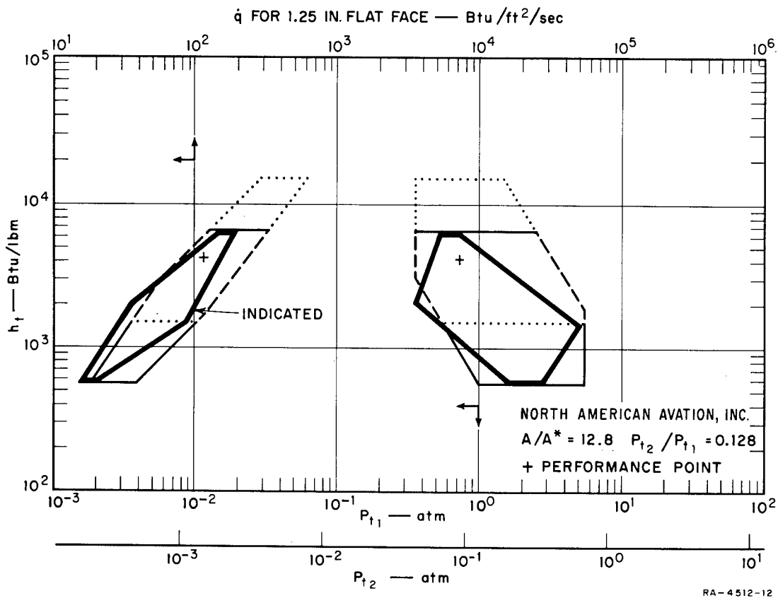
FIG. 10 ESTIMATED AND INDICATED ENVELOPES FOR NORTH AMERICAN AVIATION
