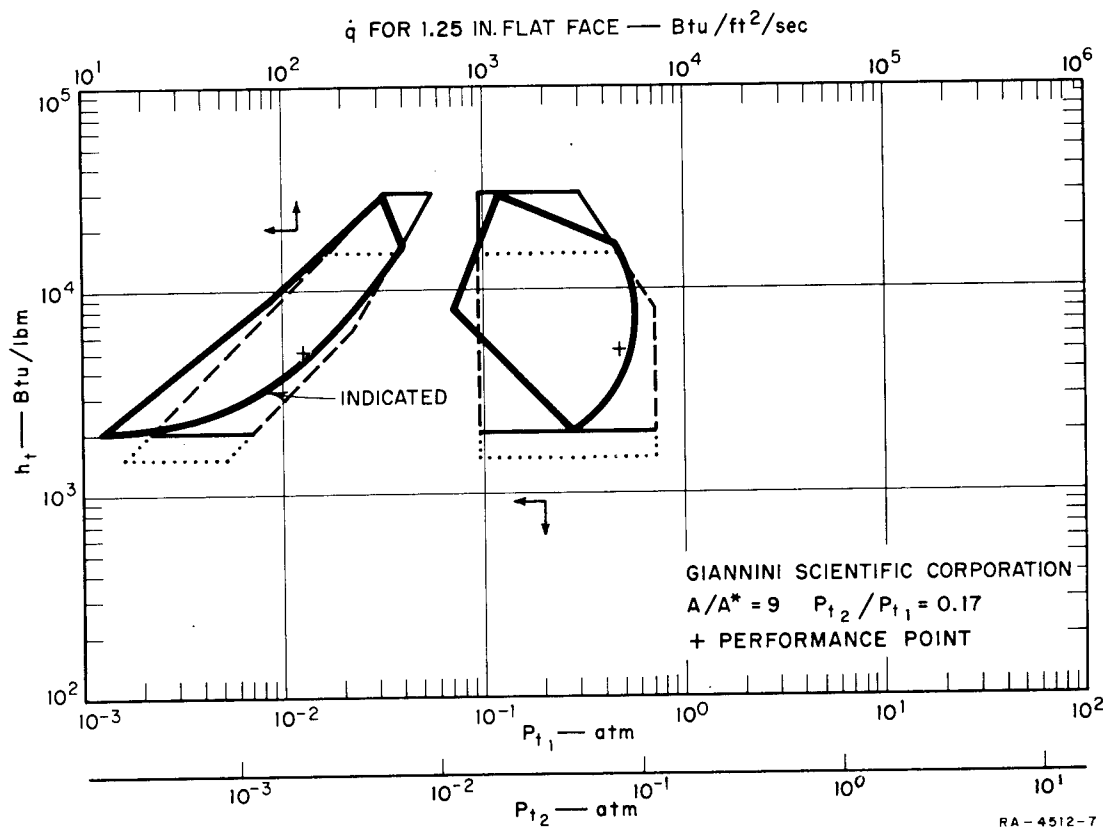
FIG. 5 ESTIMATED AND INDICATED ENVELOPES FOR GIANNINI SCIENTIFIC CORPORATION
