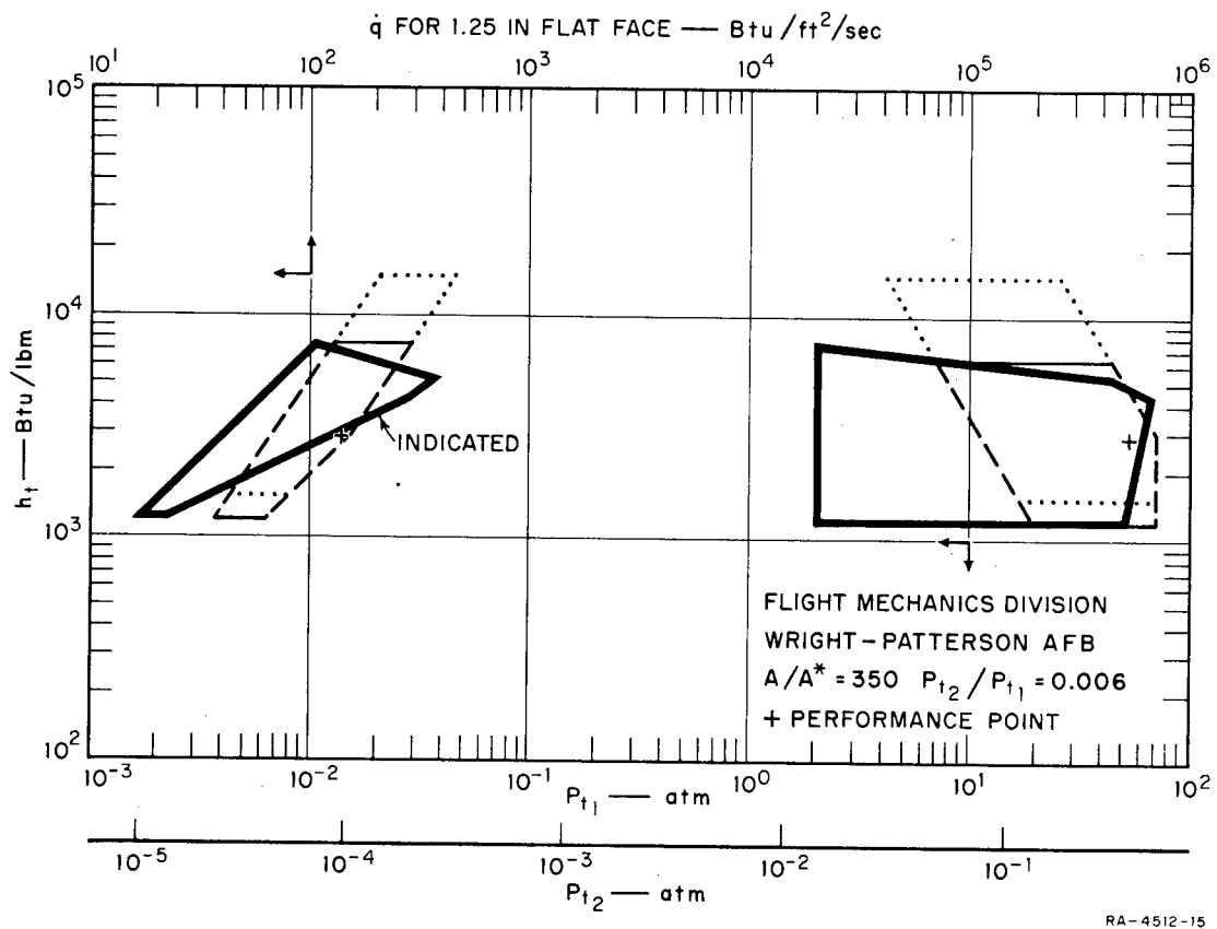
FIG. 4 ESTIMATED AND INDICATED ENVELOPES FOR FLIGHT MECHANICS DIVISION, WRIGHT-PATTERSON AIR FORCE BASE
