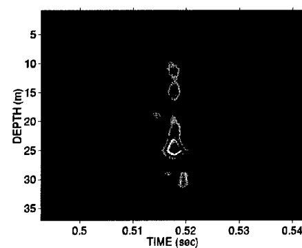
Figure 10 Example time series measured during the TR experiment. The left hand column shows a range independent focus in the Island of Elba area. The right hand column depicts a range dependent focus in the upslope region. There is more dispersion in the sloped region. Note the depth scale change on the upslope TR focus, the vertical focus is less than \pm 1 m.
