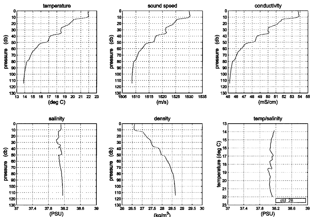
Figure 6 Sample soundspeed profile taken from the Alliance .
