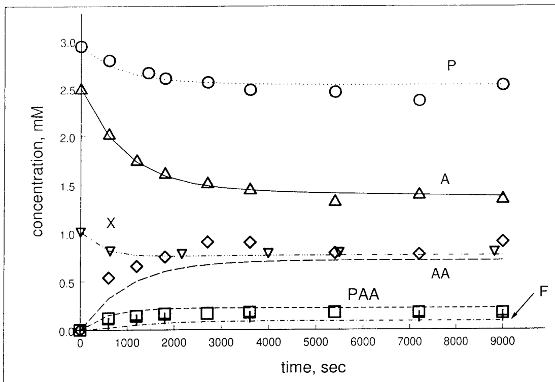
Figure 15. Concentration evolution curves for low-concentration \text{H}_2\text{O}_2/\text{UV}/\text{acetaldehyde} flow experiment with oxygen as the equilibration gas. Circles are hydrogen peroxide, triangles are acetaldehyde, inverted triangles are oxygen, diamonds are acetic acid, squares are peracetic acid, and crosses are formaldehyde. Individual symbols indicate experimental values (averaged) and lines represent predictions from kinetic model.
