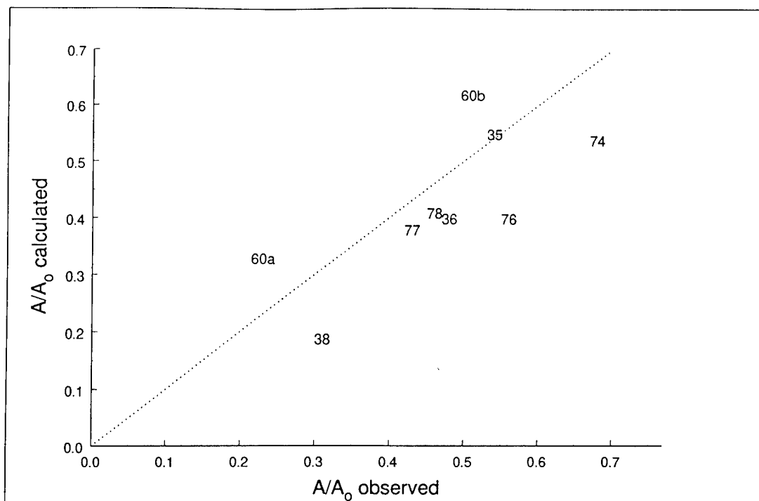
Figure 27. Comparison of experimentally determined and calculated A/A_o values for the APU and APUD series of experiments, after model calibration with both series. Symbols are experiment numbers. Line indicates region of perfect agreement.
