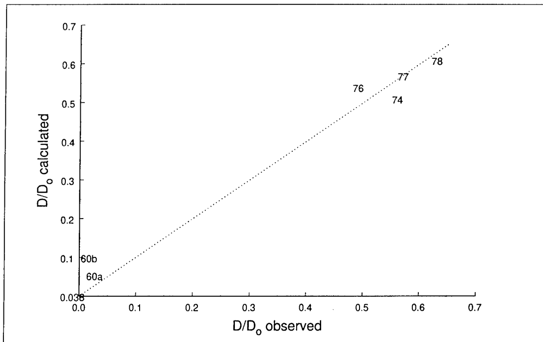
Figure 28. Comparison of experimentally determined and calculated D/D_o values for the APU and APUD series of experiments, after model calibration with both series. Symbols are experiment numbers. Line indicates region of perfect agreement.
