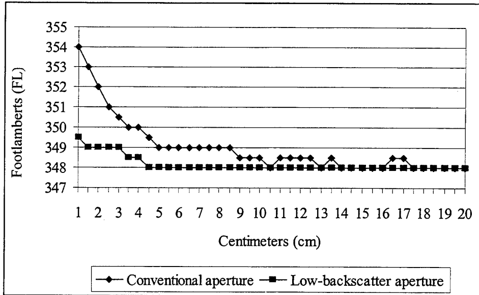
Figure 13. Comparison of lamp readings as a function of aperture distance for conventional and low-backscatter designs.
