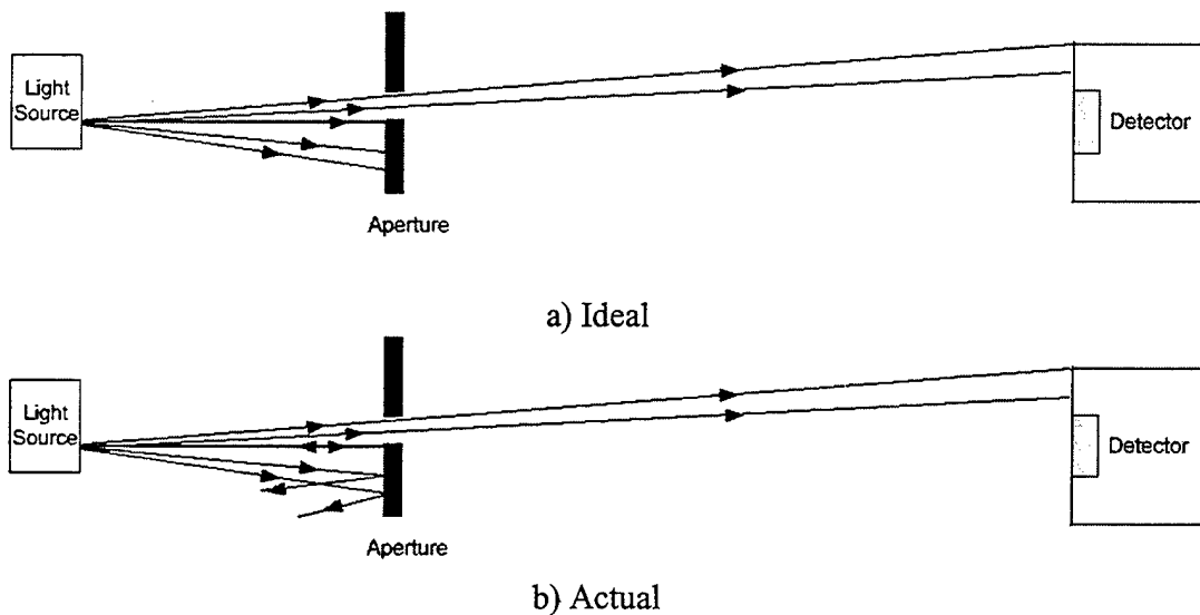
Figure 4. Ideal (top) and actual (bottom) operation of an uncollimated light source. In the actual operation, backscatter results in error (noise).
