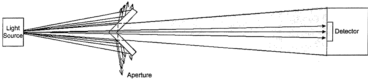
Figure 8. Illustration of the V-shaped low backscatter aperture in operation.
