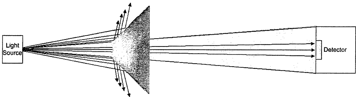
Figure 10. Illustration of the cone-shaped low backscatter aperture in operation.
