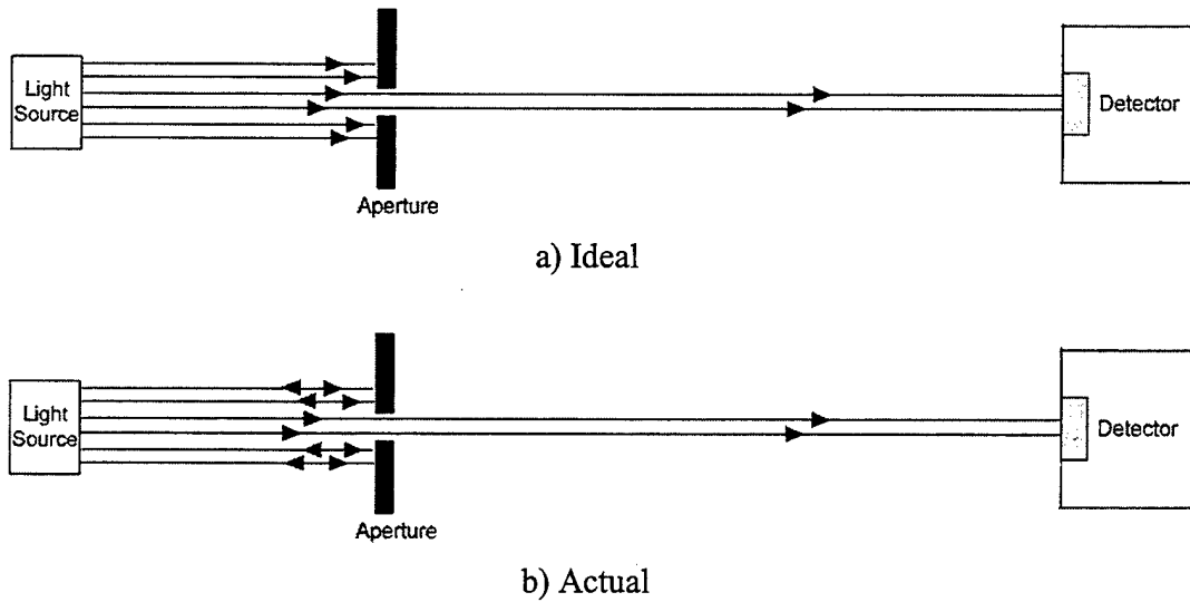
Figure 3. Ideal (top) and actual (bottom) operation of an aperture with a collimated light source. In the actual operation, backscatter results in error (noise).
