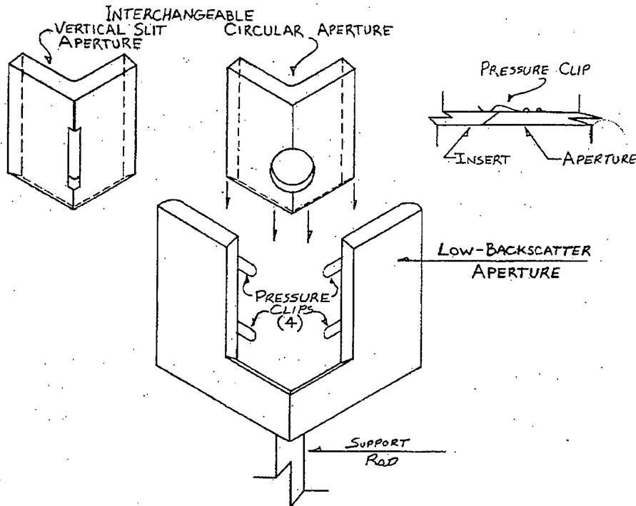
Figure 11. Concept of interchangeable aperture openings.
