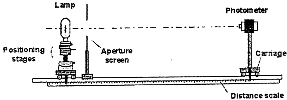
Figure 1. A simple optical system (adapted from DeCusatis, 1997).
