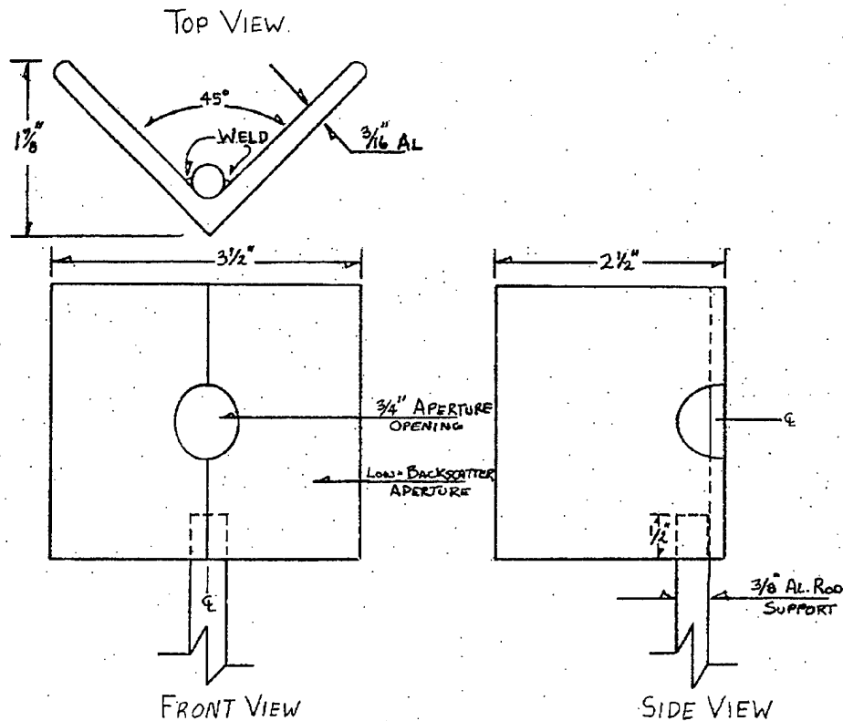
Figure 7. Basic "V"-shaped aperture design showing circular opening.
