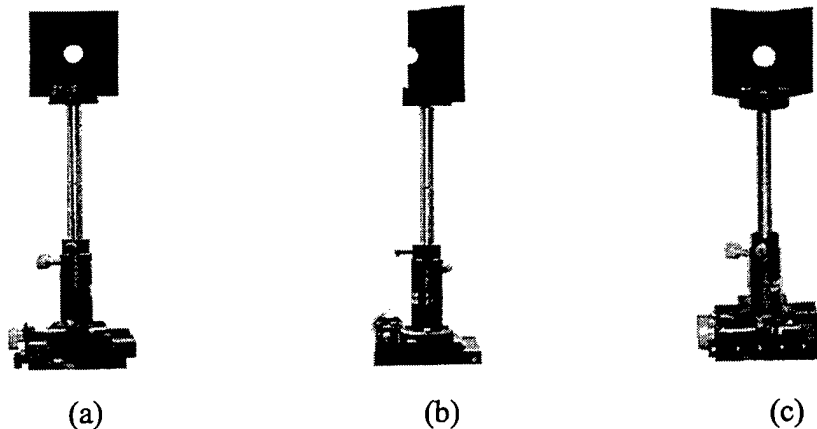
Figure 12. Front view (a) of the conventional flat aperture and side (b) and front (c) views of the low-back scatter aperture used in the concept verification measurements.
