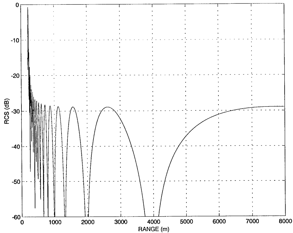
Fig. 14 — RCS with multipath, 667 reflectors above sea surface, tilted 15^\circ from perpendicular, from 0 to 1 m ( x_{\max} = 1 m; x_{\min} = 0 m; H = 59 m; tilt angle \alpha = 15^\circ ; sea state: 0 (calm); \rho = -1 ; and f = 10 GHz)
