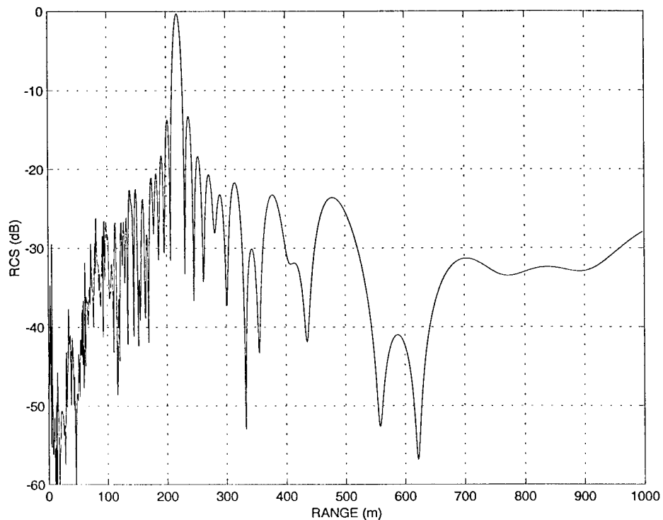
Fig. 18 — RCS without multipath, 667 reflectors above sea surface, simulating a rough reflector, tilted 15° from vertical, height from 0 to 1 m; H = 59 m; without multipath; \rho = 0 ; and f = 10 GHz
