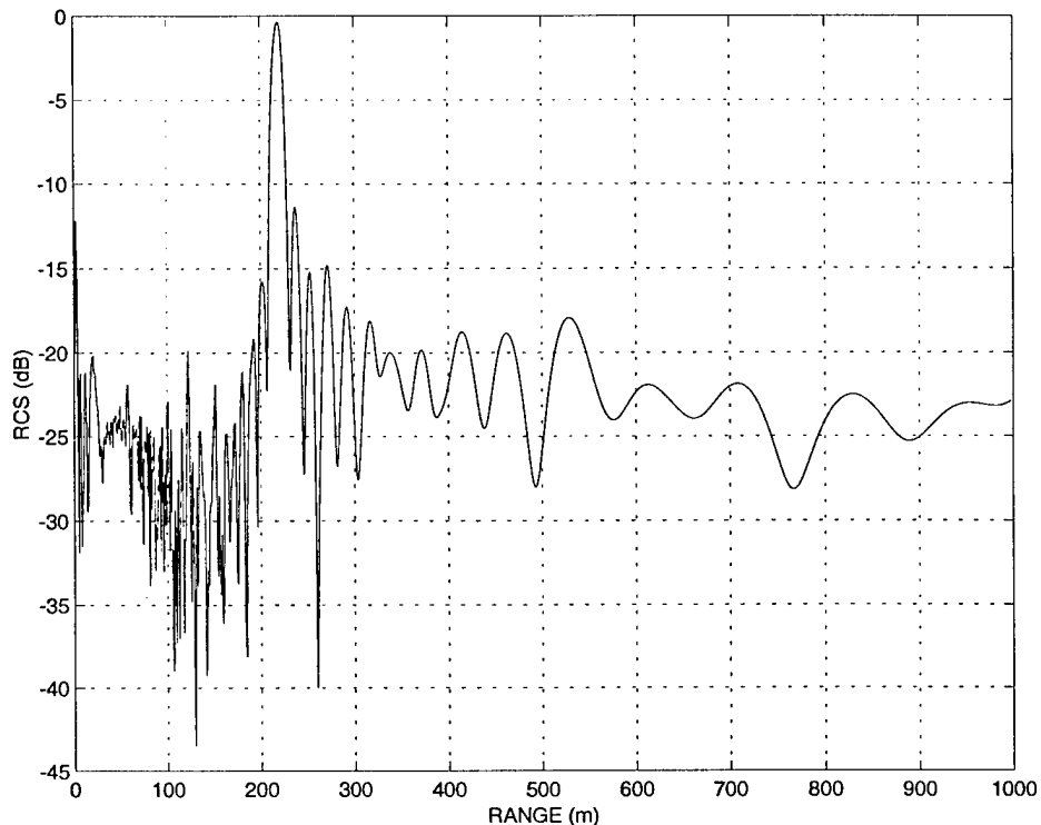
Fig. 17 — RCS with multipath, 667 reflectors above sea surface, tilted 15° from vertical, height from 0 to 1 m; H = 59 m; with multipath; \rho = -1 ; and f = 10 GHz
