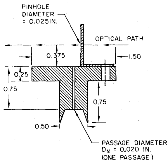
SIDE SECTIONAL VIEW AT A-A
