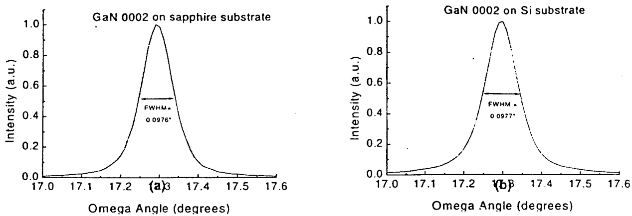
Figure 1: Comparison of GaN film quality by x-ray rocking curve of the 0002 GaN reflection for: (a) GaN on sapphire, and (b) after transfer from sapphire to a Si substrate. The FWHM of the 0002 GaN reflection remains unchanged after lift-off indicating that the film was separated and transferred without appreciable thermal or mechanical damage. A laser fluence of 600 mJ/cm 2 was used.
