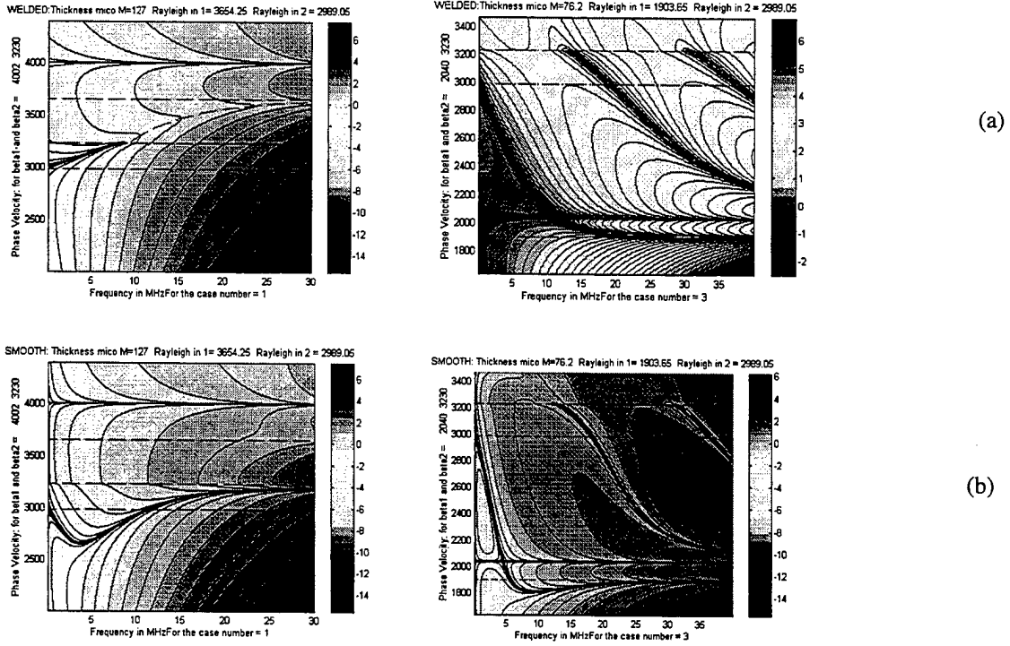
Figure 3. Theoretical phase velocity dispersion contours calculated from the experimental parameters for the following cases: coating acoustically more stiff (left) and less stiff than the substrate (right), welded contact (a), and smooth contact (b). Note: the 1 and 2 refer to the Rayleigh velocities of the layer and substrate, respectively.
