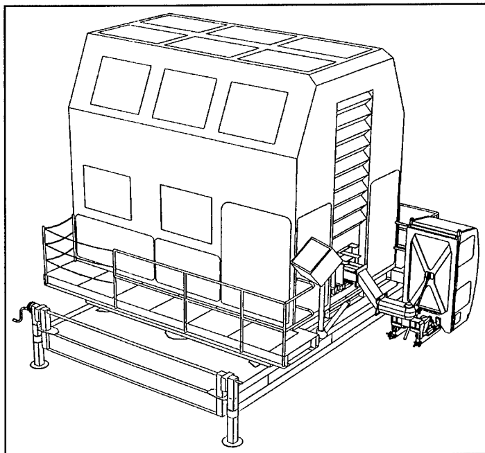
Figure 2-8. Rack Insertion Device
