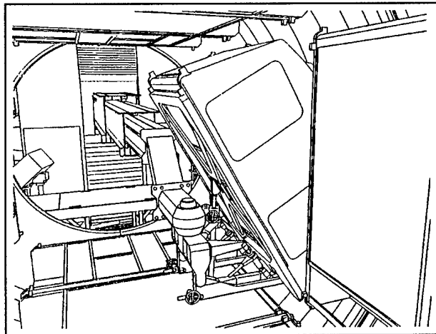
Figure 2-9. Rack Installation
