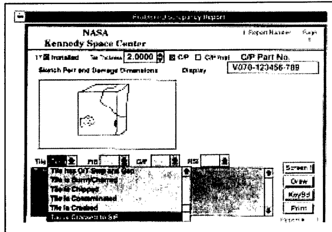
Figure 2-6. Draw Screen
