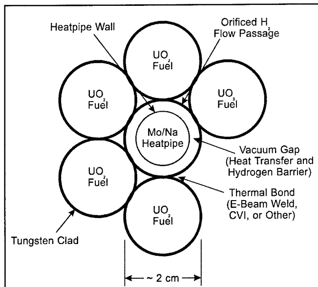
Figure 3-4. Heatpipe Bimodal System 5-pin Module
