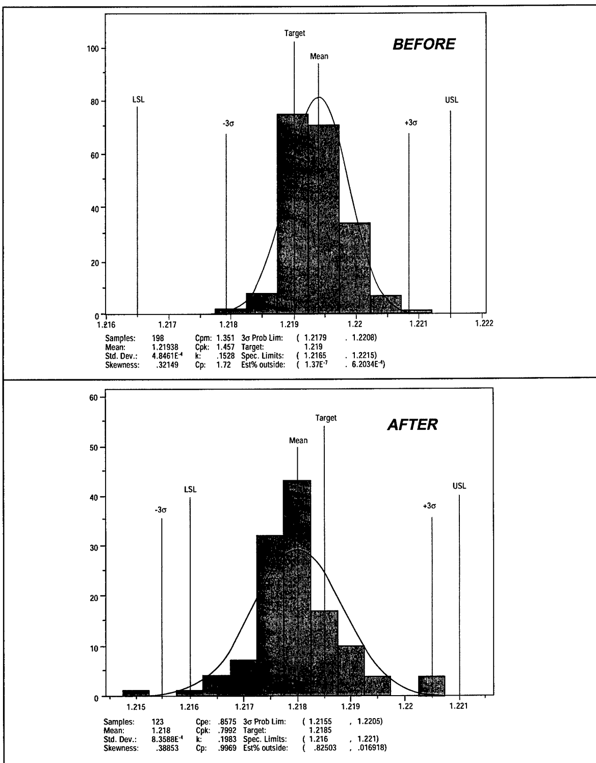
FIGURE 3-1. PROCESS CAPABILITY (FOR OVERALL LENGTH PARAMETER OF ELECTRICAL CONTACT) BEFORE AND AFTER SPC
