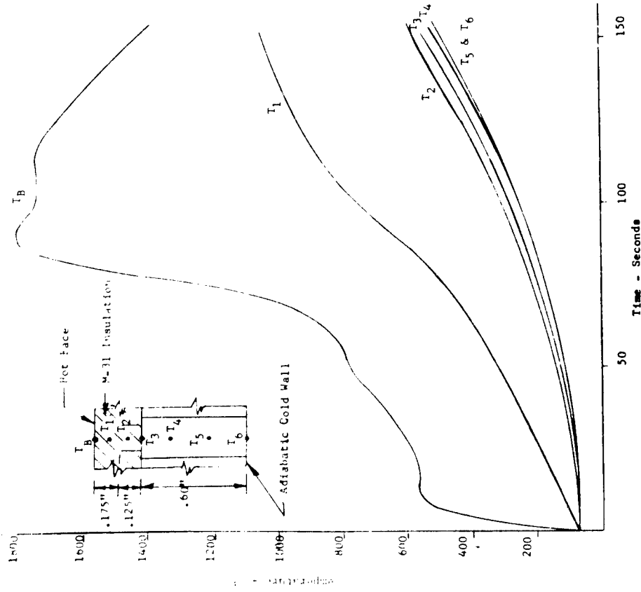
Figure 18 Temperature Profiles -- Panel Sk 60B20001 .015 Inch Node Flow Width - Cell Size 4-15 Open Core Size, 8-15
