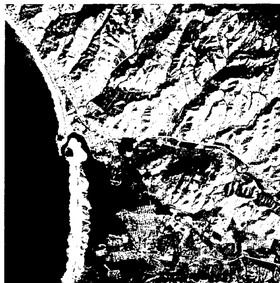
Figure 2. (a) False Color composite of Moro Bay (Red = band 4, Green = band 3, Blue = band 2.) (b) True color composite image (Red = band 3, Green = band 2 and Blue = band 1.) 2
