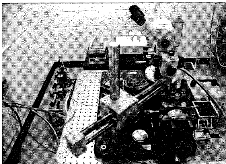
Figure 6. Viewing port of the Cryogenic System with Microscope Installed.
