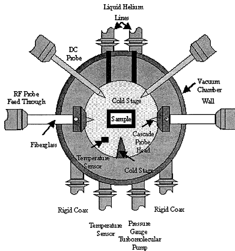
Figure 5. Top View of Cryogenic Measurement Chamber.
