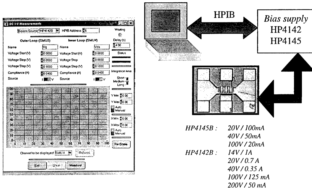
Figure 1. Schematic of a DC-IV System.
