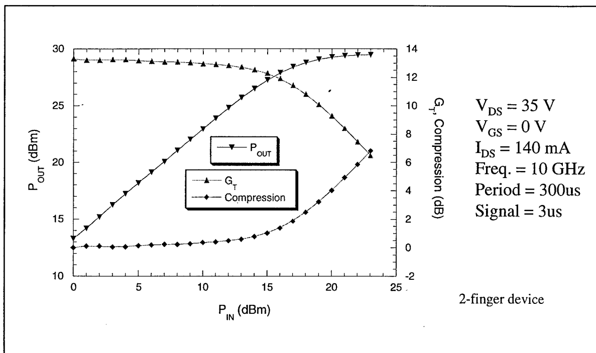
Figure 31. Output Power, Gain and Gain Compression at V_{GS} = 0 Volts.
