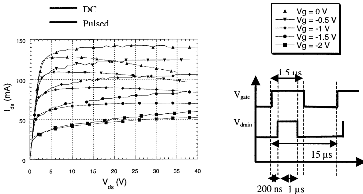
Figure 3. Difference Between DC-IV and Pulsed-IV Characteristics at Room Temperature.
