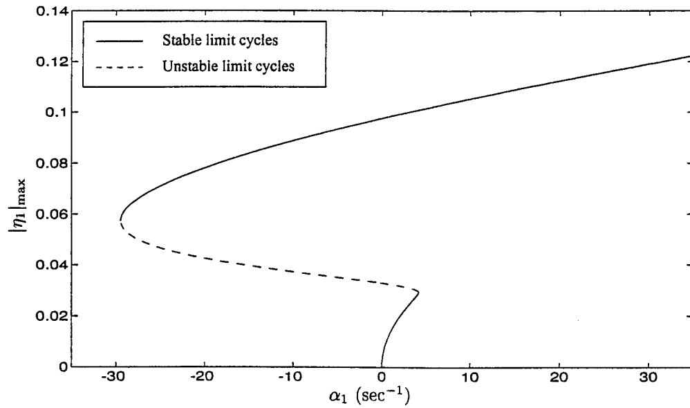
Figure 10: Bifurcation diagram for the deterministic system; threshold velocity model, u_t/\bar{a} = 0.03 , R_{vc} = 7.8 , 4 modes
