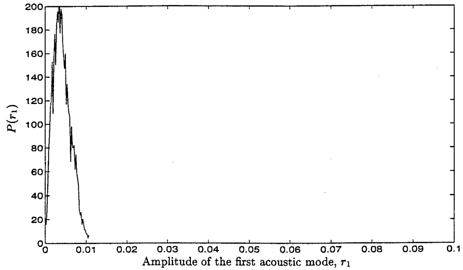
Figure 2: The influence of an external excitation of the fundamental mode only on a linearly stable system; 2 modes, \sigma_1^E = 0.0005 \text{ sec}^{-3/2} , \alpha_1 = -25 \text{ sec}^{-1}
