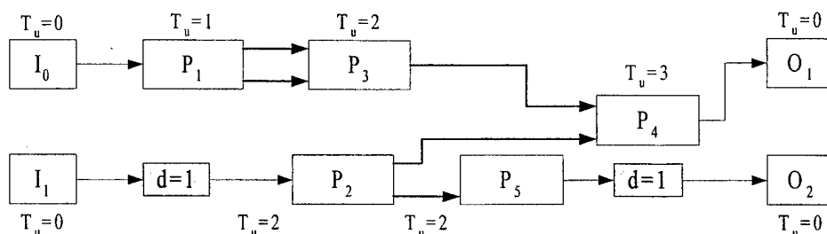
Figure 12. An Optimum Synchronization of Figure 11
