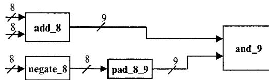
Figure 9. Insertion of a "Padding" Module
