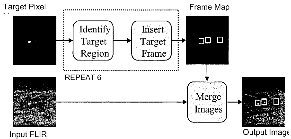
Figure 18. An Internally Developed ATR Algorithm
