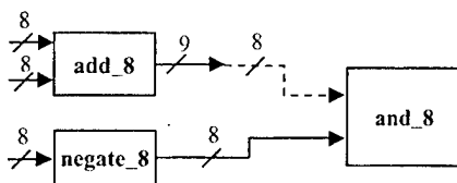
Figure 6. A Positively Mismatched Data Path
