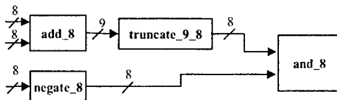
Figure 7. Insertion of a “Truncating” Module.
