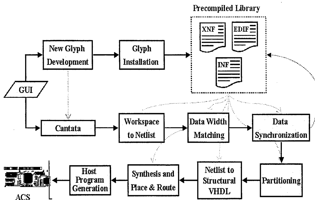
Figure 3. Overview of the CHAMPION Design Flow
