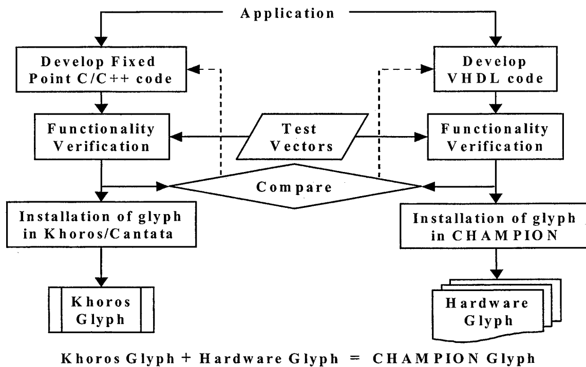
Figure 4. Steps for Developing a New Module
