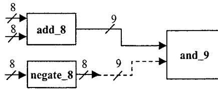
Figure 8. A Negatively Mismatched Data Path
