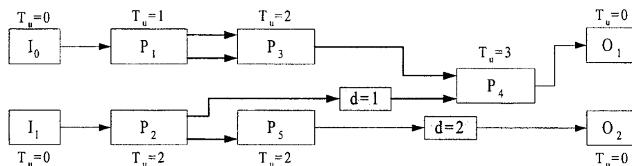
Figure 11. Synchronization Using the Straightforward Approach
