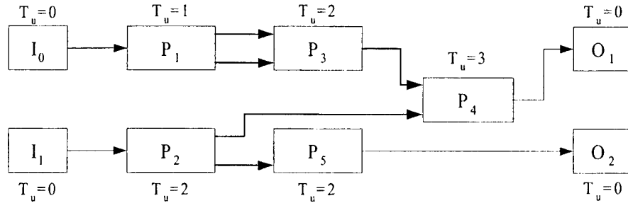
Figure10. An Unsynchronized Digital System
