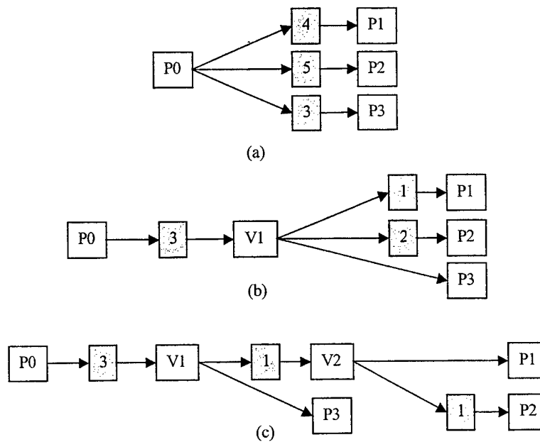
Figure 15. Delays of the Hyper-Arc
