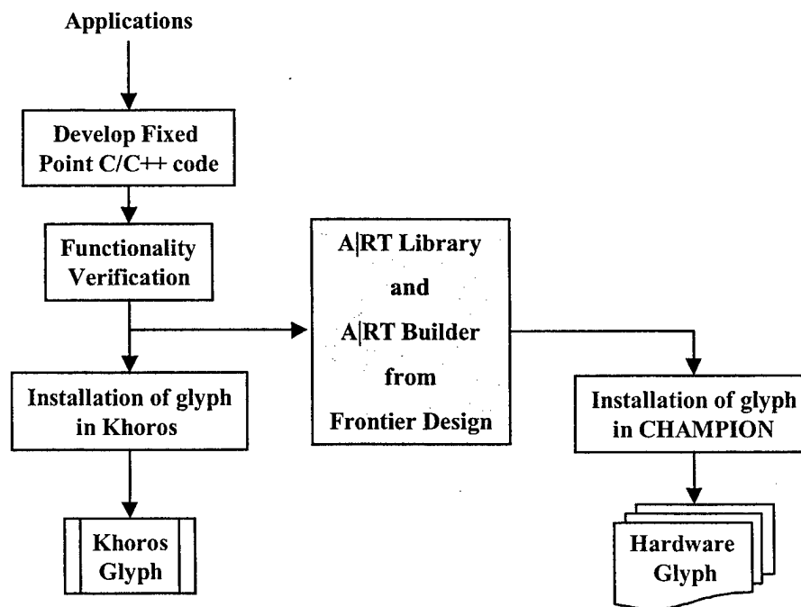
Figure 5. New Module Development Using A|RT tools
