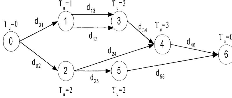
Figure 13. The SFG Representation of the Digital System Shown in Figure 10
