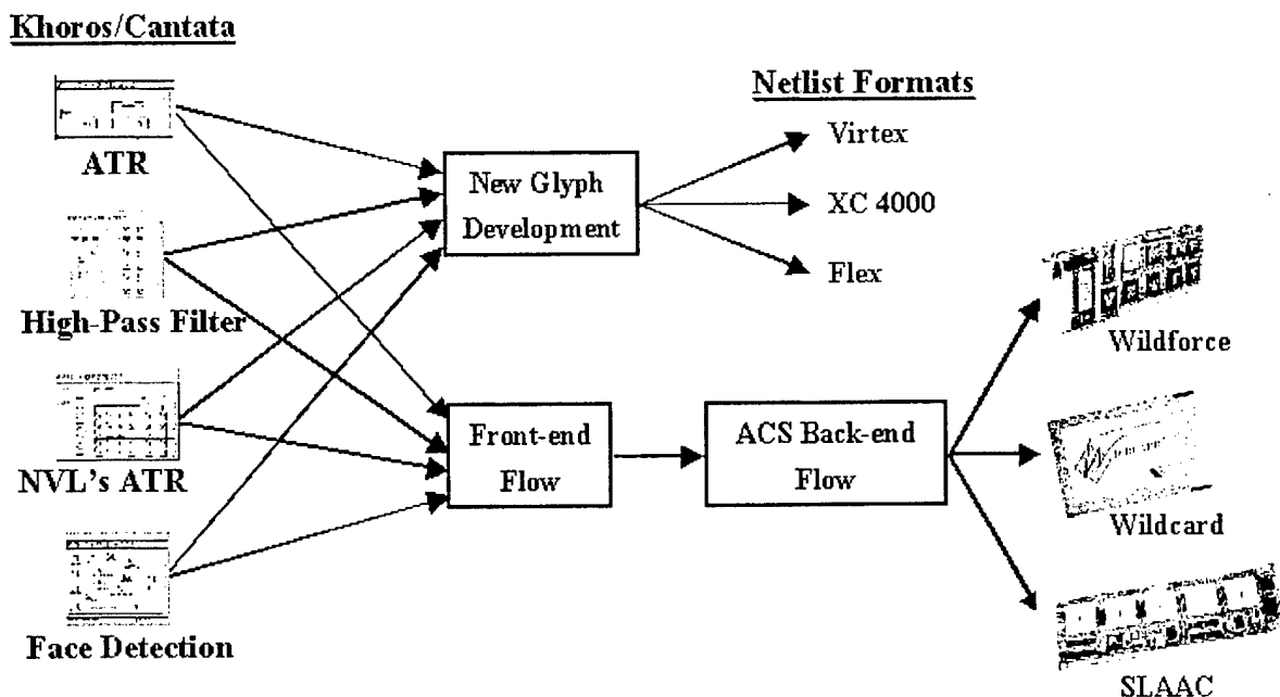
Figure 16. Mapping onto Multiple ACSs
