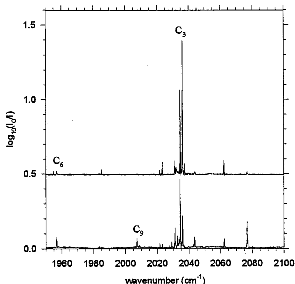
Figure 6. IR Absorptions of Carbon Clusters in pH 2 at T = 2 K. The sample was prepared by laser ablation of graphite. The top trace shows the as-deposited sample, with: T = 2 K, \lambda_{\text{abl}} = 308 nm, \Phi_{\text{abl}} \approx 8 \times 10^7 W/cm 2 , 100 mJ/pulse, 10 Hz repetition rate, 30 minute C n deposition time, H 2 inlet flow rate \approx 120 mmol/hr, l = 1.2 mm. The bottom trace shows the sample again at 2 K, after warming to 4 K. Resolution is 0.15 cm -1 FWHM.
