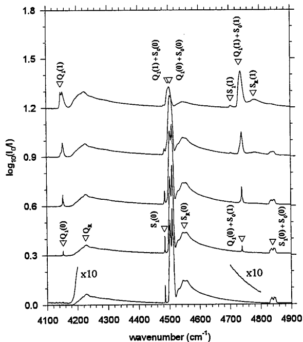
Figure 3. Ortho/para composition of \approx 0.9 mm total (front + back) thickness vapor deposited solid hydrogen samples at T = 2 K. The oH_2 concentrations increase from bottom to top in the sequence: 0.01%, 2%, 8%, 25%, and 70%, corresponding to o/p converter bobbin temperatures of: 15 K, 28 K, 37 K, 52 K, and 135 K. In each case \approx 55(\pm 3) mmol of hydrogen were deposited in a 1 hour period. The absence in the bottom trace of the Q_1(0) ( 4153 \text{ cm}^{-1} ) and Q_1(0)+S_0(1) ( 4740 \text{ cm}^{-1} ) absorptions is evidence of the very low oH_2 concentration ( < 0.1\% ) in that sample. The spectra are presented at 1 \text{ cm}^{-1} FWHM resolution.
