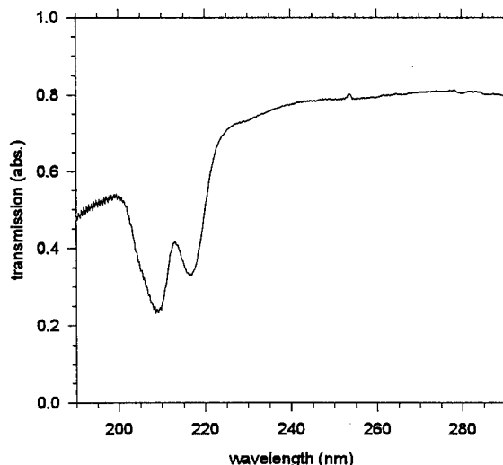
Figure 7. UV Transmission Spectrum of B/H 2 at T = 2 K. The sample was prepared by laser ablation of solid boron with: T = 2 K, \lambda_{\text{abl}} = 308 nm, \Phi_{\text{abl}} \approx 9 \times 10^7 W/cm 2 , 110 mJ/pulse, 10 Hz repetition rate, 60 minute B deposition time, H 2 inlet flow rate \approx 55 mmol/hr, l = 1.0 mm.
