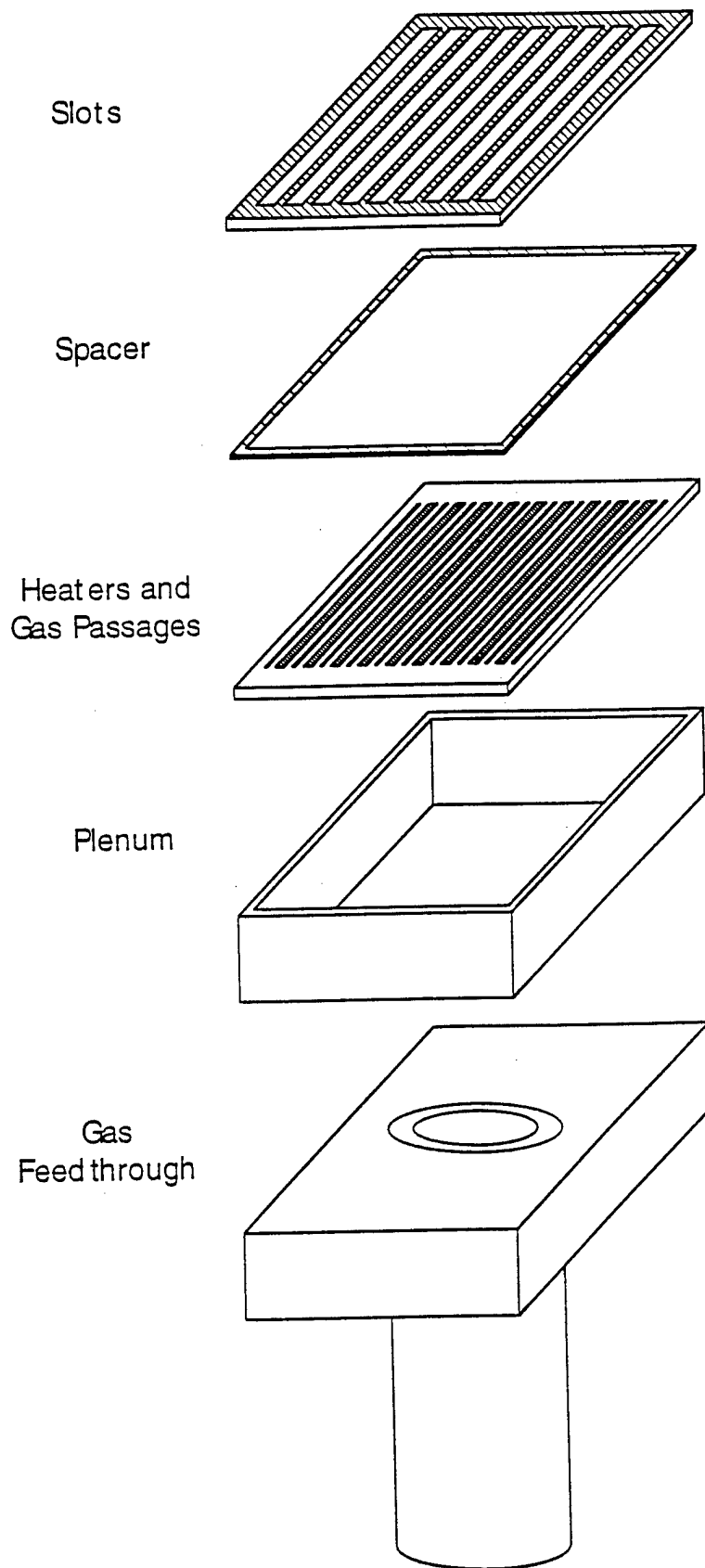
Figure 4: Exploded view of the FMVR.
