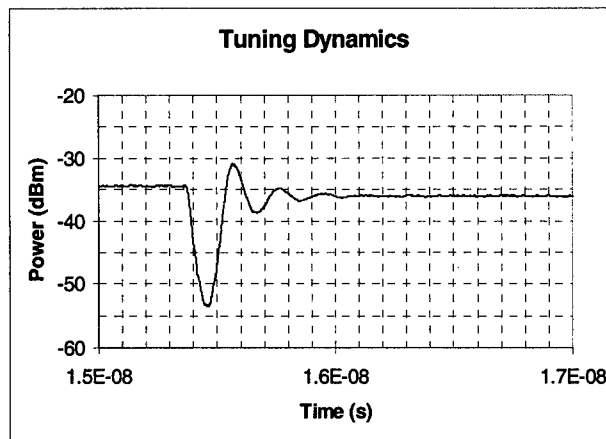
Figure 36. 500 ps tuning of a laser with a bias current of 50 mA and a differential gain of 3.0 \times 10^{-20} \text{ cm}^2 .
