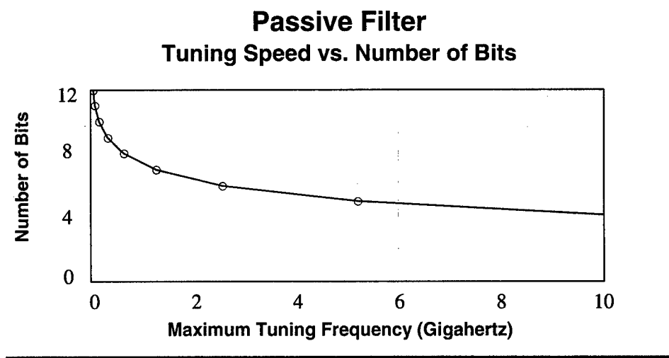
Figure 19. Tuning speed vs. number of bits for passive filter.
