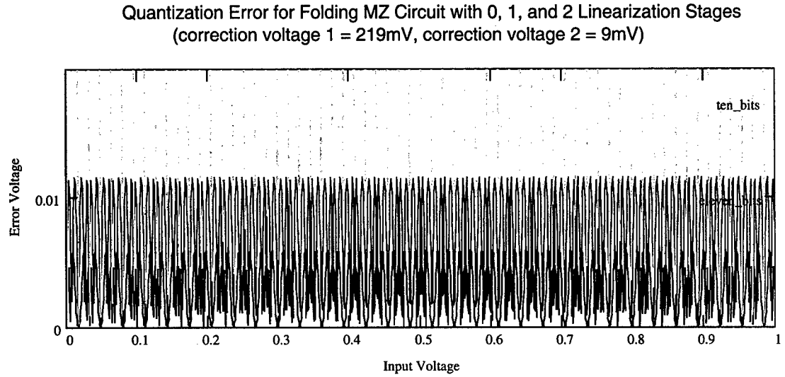
Figure 7. One and two term linearization system simulation results.
