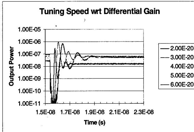
Figure 35. Tuning characteristics as a function of differential gain of the SOA in the range of 30 to 100 mA.
