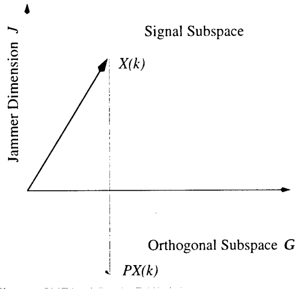
Fig. 1 Jammer suppression by subspace projection.
