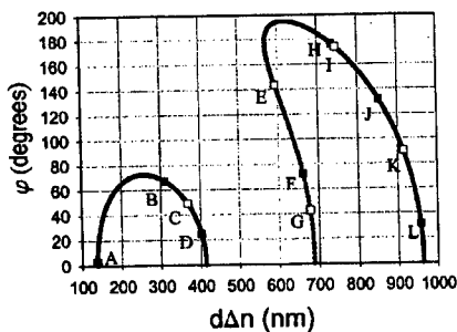
Fig. 3. Optimum conditions for the RBTN structure. The solid circles are the optimum conditions for perpendicular SOP output. The squares are the optimum conditions for both of the bistable states. The open squares indicate that the other state has a twisted angle \varphi + 2\pi ; the filled squares indicate that the other state has a twisted angle \varphi - 2\pi .
