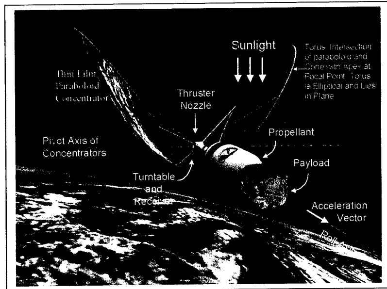
Figure 1. Solar Thermal Propulsion Rocket AFRL
