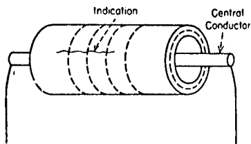
-Circular Magnetization, Current Through a Conductor.
