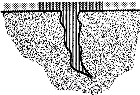
Developer acts like a blotter to draw penetrant out of crack.
