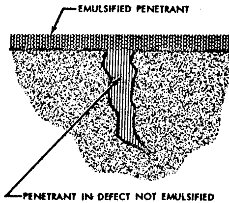
Penetrant on surface and emulsifier are mixed.
