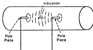
-Circular Magnetization with "Prod" Type Contacts.
