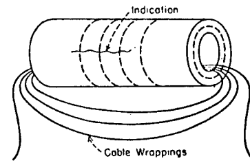
-Circular Magnetization, Current Through Conductors Threaded Through Forging.
