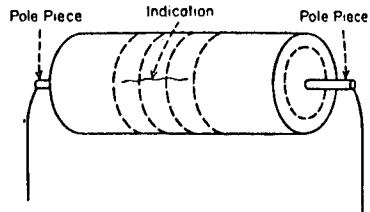
-Circular Magnetization, Current Directly Through Forging.
