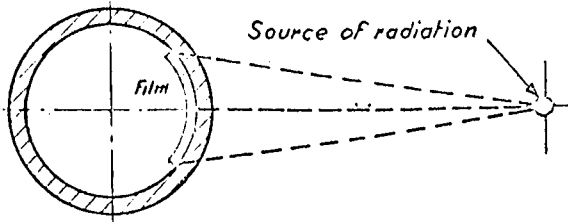
Method A — Film inside, radiation source outside
