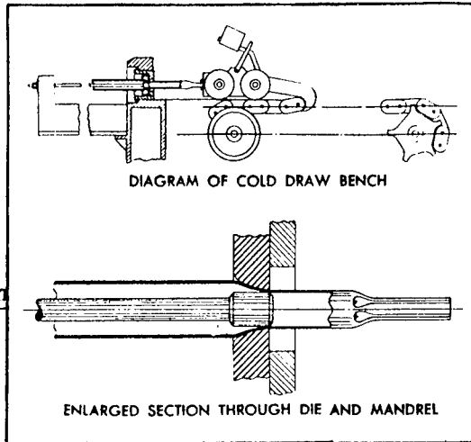
Fig. 5 Cold Drawing Operation
