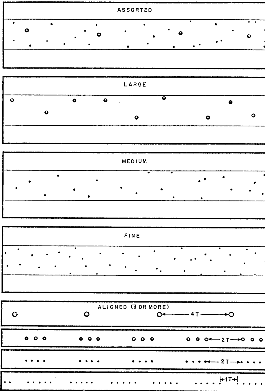
PLATE OVER \frac{1}{4} IN. TO \frac{1}{2} IN.
