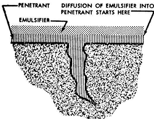
Emulsifier applied to penetrant.
