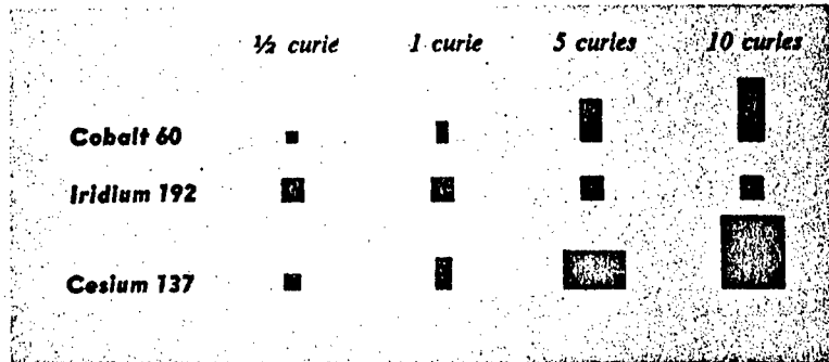
Fig. 6 - Comparison of Physical Dimensions of Typical Gamma Ray Sources of Equal Size (in Curies).
