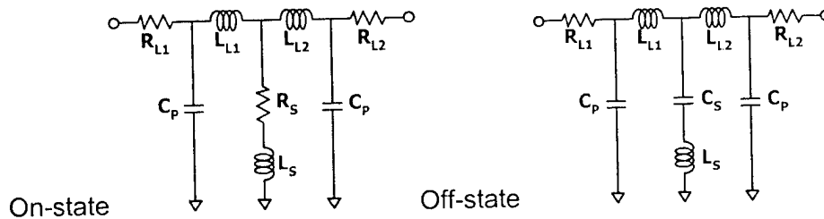
Figure 14: Simplified circuit model of the switch in on and off states.
