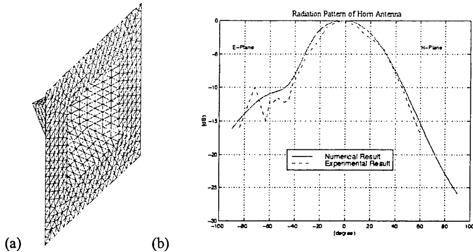
Figure 1: (a) Meshed model of a micromachined horn antenna; (b) spatial distribution of RF radiation simulated using the frequency-domain simulation tools.
