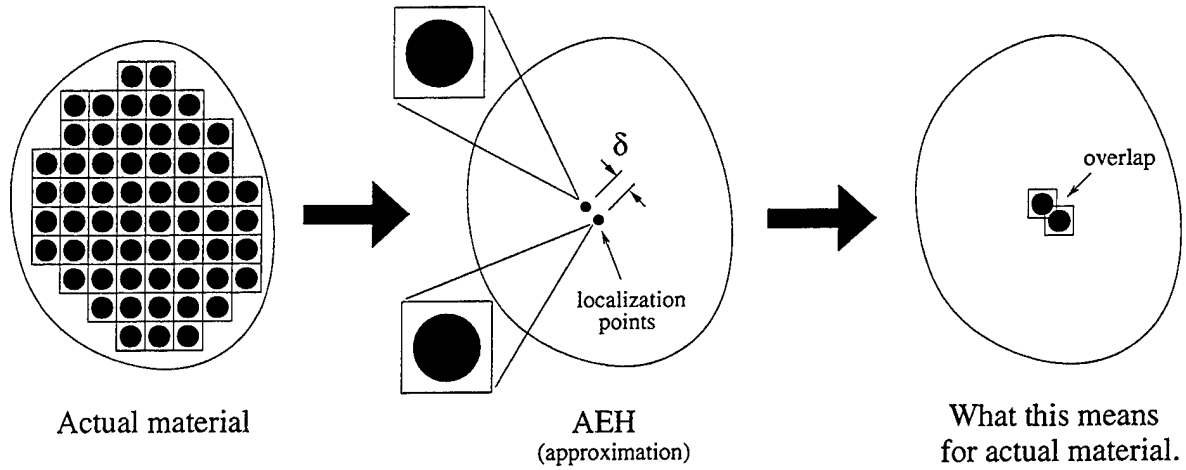
Figure 12. The single-point localization paradox. The approximations of the AEH approach remove length scale information at the microlevel. This allows for unit cells to overlap conceptually and leads to the localization paradox.
