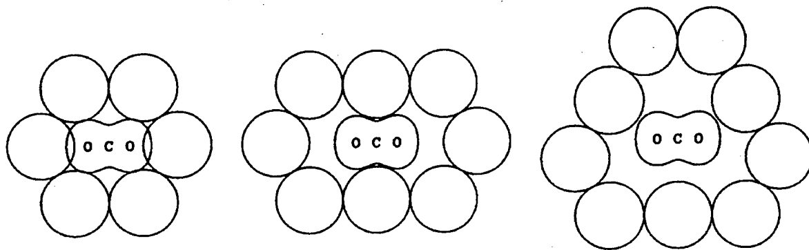
Figure 4. Hypothetical trapping sites for CO 2 molecules in solid pH 2 based on single-, double-, and triple-substitutional vacancies in close-packed planes of pH 2 molecules.
