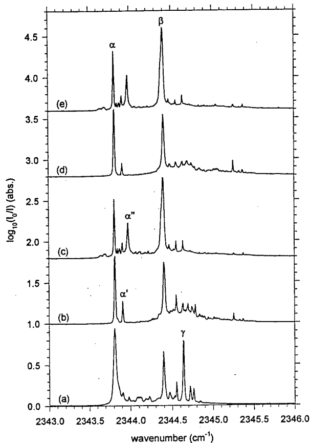
Figure 2. Annealing behavior of the 1.2 PPM \text{CO}_2/\text{pH}_2 sample described in figure 1. Trace (2a) is an expanded view of the as-deposited spectrum presented above in trace (1c). The temperature sequence is: (2a) T = 2.4 K, (2b) T = 4.8 K, (2c) T = 2.4 K, (2d) T = 4.8 K, and (2e) T = 2.4 K. The labels \alpha' and \alpha'' denote two new features that grow in during annealing.
