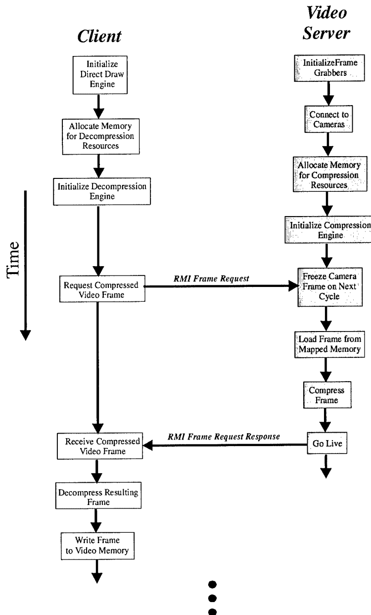
Figure 9.1-2. Video Server communications protocol.
