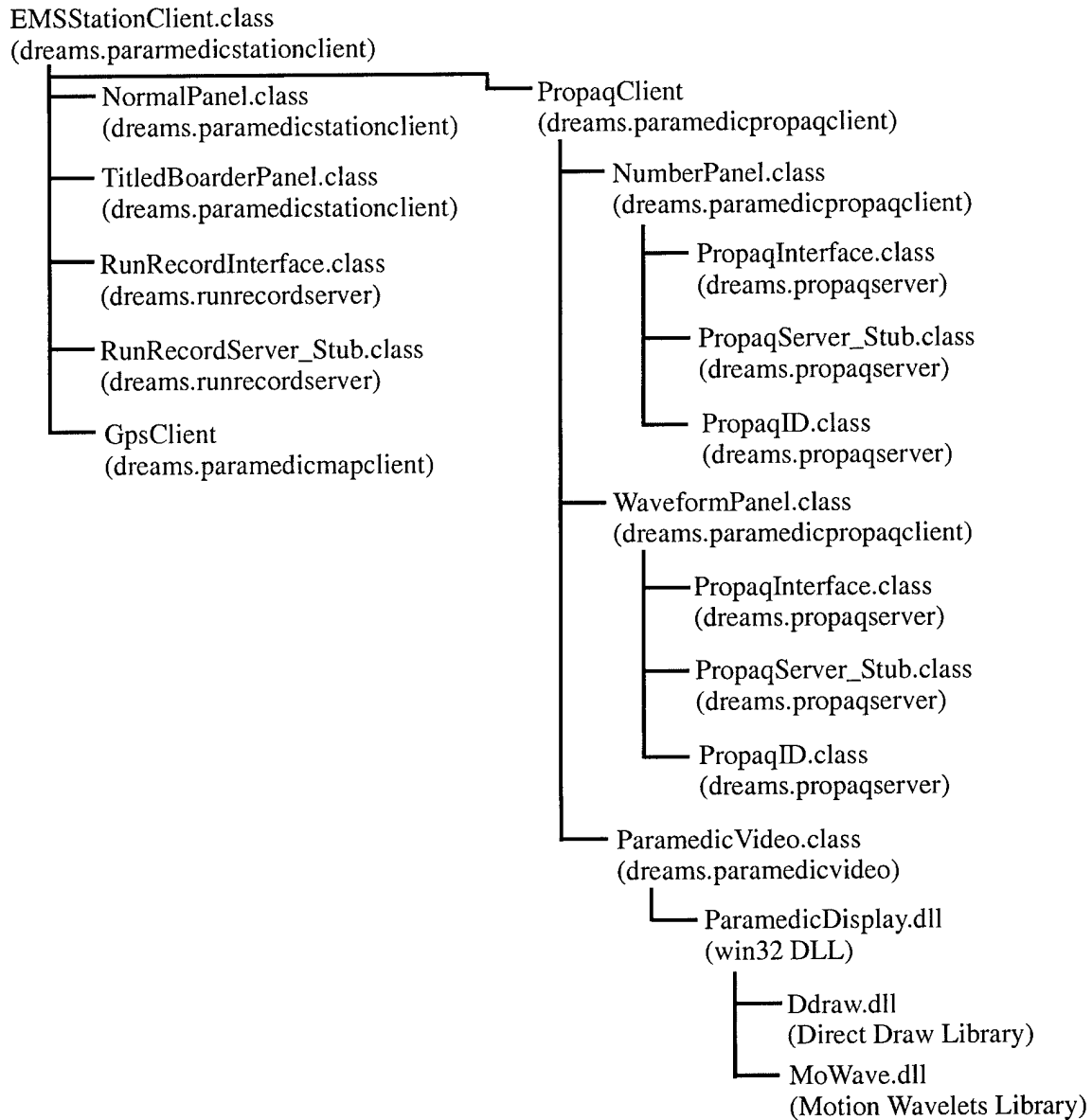
Figure A-3. Paramedic-Mobile Station Client dependency graph (continued).
