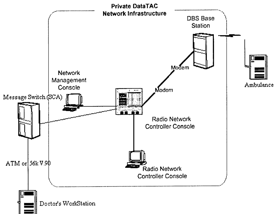
Figure 12.4.2-1. Motorola DataTAC 2.0 RF Infrastructure.
