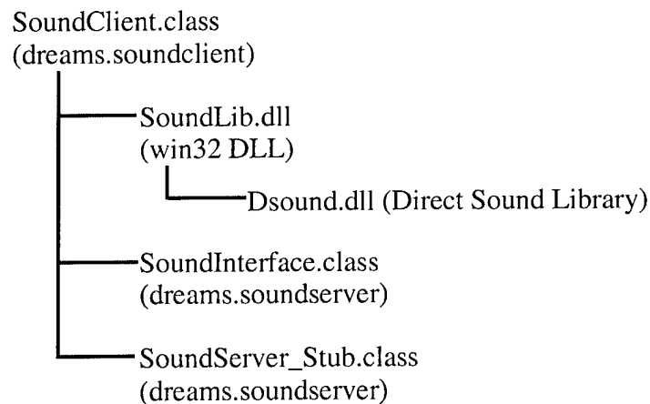
Figure A-4. Dependency graph for Sound Client Java class.
