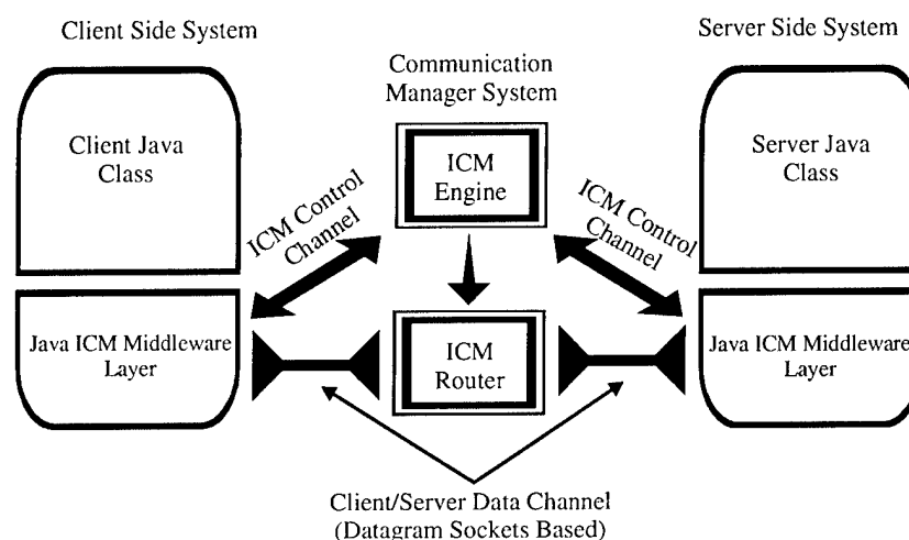
Figure 12.5-1. ICM module components.
