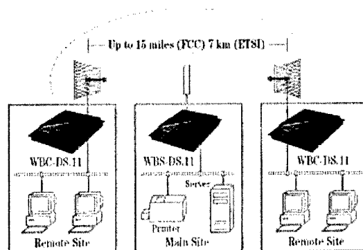
Figure 12.4.3-1. BreezeCom RF infrastructure.
