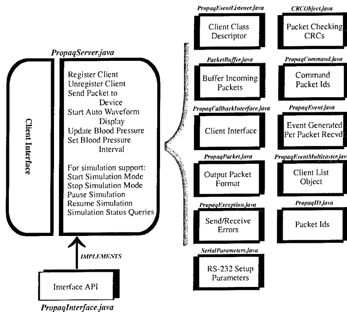
Figure 9.3-1. Propaq Server components in system.
