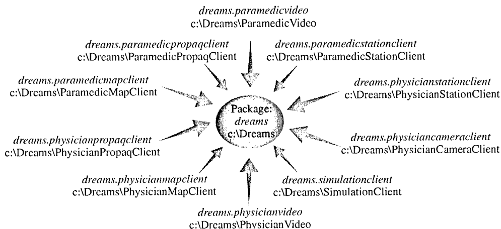
Figure 5-2. Client packages for the Digital EMS software modules.
