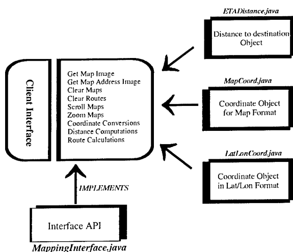
Figure 9.7-1. Map Server components in system.
