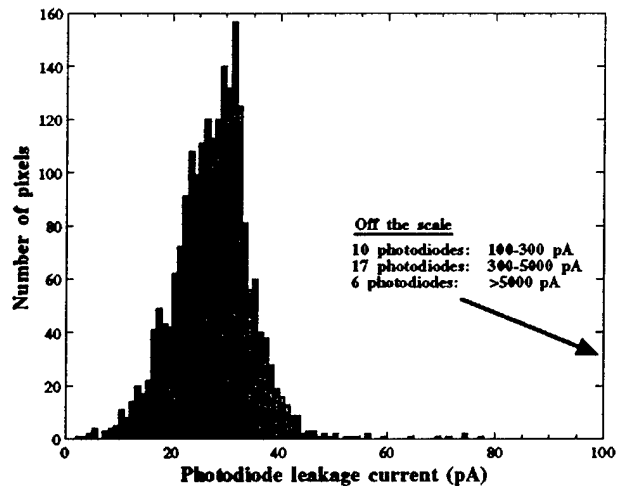
Fig. 3. Histogram of the leakage current values for photodiodes in 34 64-pixel arrays. Histogram bins are 1 pA wide. Photodiodes are 3 mm × 3 mm in size and were in the dark at room temperature under a 50 V bias. The pixels with leakage current less than 100 pA (2143 out of 2176) demonstrate an average current of 28 \pm 7 pA.
