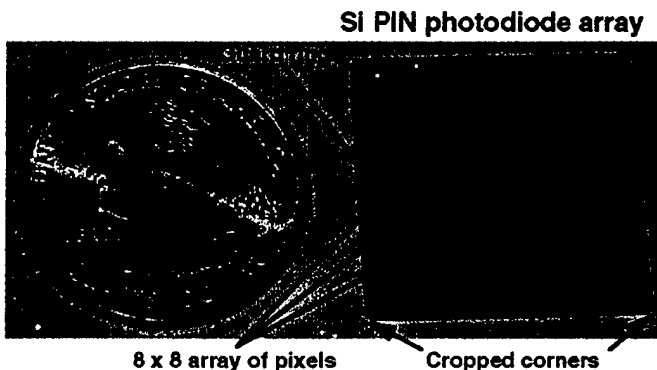
Fig. 2. Low-noise Si PIN photodiode array consisting of 64 3 mm × 3 mm pixels, with a quarter (2.4 cm diameter) for scale. The side shown in the patterned n-layer, while the backside is the unpatterned, light-sensitive n-layer. A series of 4 guard rings encircle the array of pixels.
