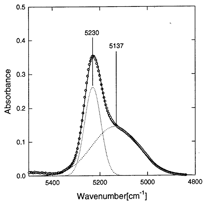
Figure 2.16. Deconvolution of the 5400-4800 \text{cm}^{-1} range after 13-day exposure. Two separate processes were described by Gaussian function.
