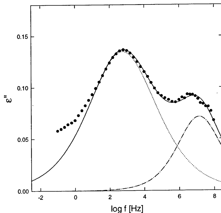
Figure 2.5. Dielectric loss in the frequency domain after 5-day exposure to environment, measured at -30^{\circ}\text{C} . \beta and \gamma processes were fit to the Cole-Cole equation.
