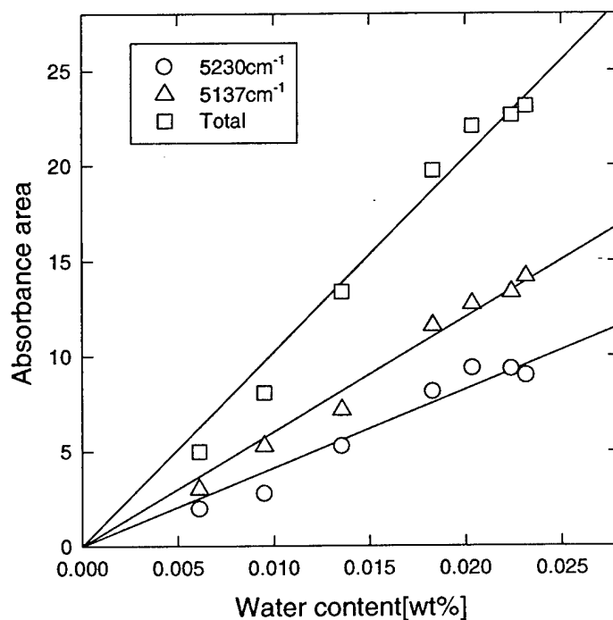
Figure 2.17. Absorbance area as a function of water content for absorbances of 5230 \text{cm}^{-1} , 5137 \text{cm}^{-1} , and their sum.
