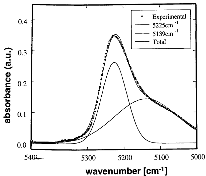
Figure 3.15. Deconvoluted difference spectra in the 5000-5400 cm -1 range after a 4-day exposure to 60°C /98 %RH.
