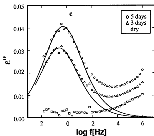
Figure 3.7. Dielectric loss in the frequency domain for cured BMI exposed to 60°C/98% RH with exposure time as a parameter, measured at (a) -20°C, (b) -60°C and (c) -100°C.
