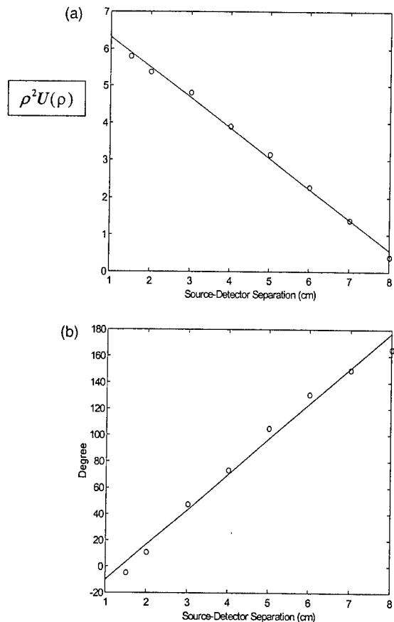
Fig. 4. Calibration curves. (a) \log [\rho^2 U(\rho)] versus source-detector separation. (b) Phase versus source-detector separation.
