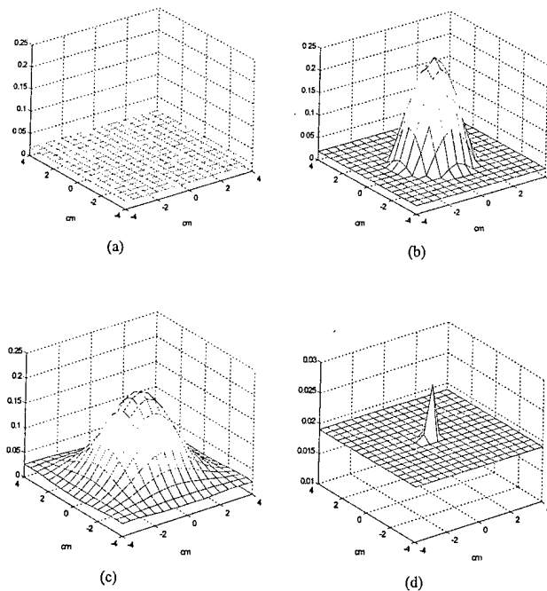
Fig. 7. Simulated 3-D images of \hat{\mu}_\alpha reconstructed with a total of 28 \times 13 = 364 source-detector pairs. The target ( \mu_\alpha = 0.25 \text{ cm}^{-1} ) was located at ( x = 0, y = 0, z = 3.0 \text{ cm} ) inside the Intralipid background. (a) Reconstructed \hat{\mu}_\alpha at nontarget layer 2 (simulation, 0.5% noise). No image lobe was observed. (b) Reconstructed \hat{\mu}_\alpha at target layer 3 (simulation, 0.5% noise). The target of strength \hat{\mu}_{\alpha(\text{max})} = 0.248 \text{ cm}^{-1} and the spatial location (0.0, 0.0) was observed. (c) Reconstructed \hat{\mu}_\alpha at nontarget layer 4 (simulation, 0.5% noise). The target of strength 0.190 \text{ cm}^{-1} and location ( x = 0.0, y = 0.0 ) was observed. (d). Reconstructed \hat{\mu}_\alpha at nontarget layer 2 with 1.0% noise. The target of 0.028 \text{ cm}^{-1} was observed. Note that the scale of (d) is different from (a)-(c).
