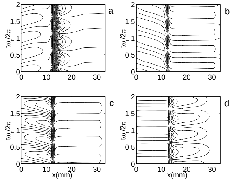
Figure 7.4: Mode 1: Contour plots of (a) n_1 , (b) \Gamma_{i1} , (c) \Gamma_{e1} , and (d) \phi_1 .
