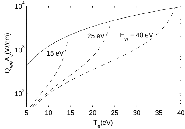
Figure 4.9: Energy losses per unit of channel length for different wall materials, A_c = 40 \text{ cm}^2 , d = 15 \text{ mm} , \hat{n}_e = 10^{18} \text{ m}^{-3} , and \tilde{\nu}_w = 1 . The solid line corresponds to the CSR. Energy losses are proportional to \tilde{\nu}_w .
