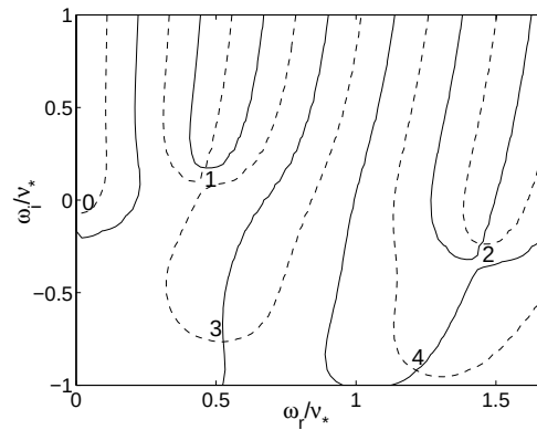
Figure 7.1: First self-excited modes for the stationary solution of Fig. 3.2. Solid lines: D_{re} = 0 ; dash-dot lines: D_{im} = 0 . Modal frequencies are given by the intersection of both lines. Dashed lines are contour lines for |D| constant and small.
