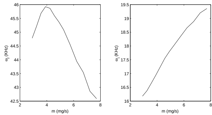
Figure 7.11: Evolution of the complex frequency of Mode 1 with \dot{m} . The rest of 0th order parameters as in Fig. 3.2.
