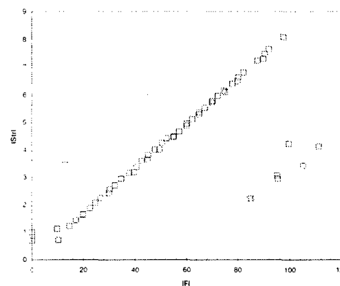
Fig. 11b. Strouhal number variation with excitation frequency. Angle of attack: 10°; leading edge flap actuation.
