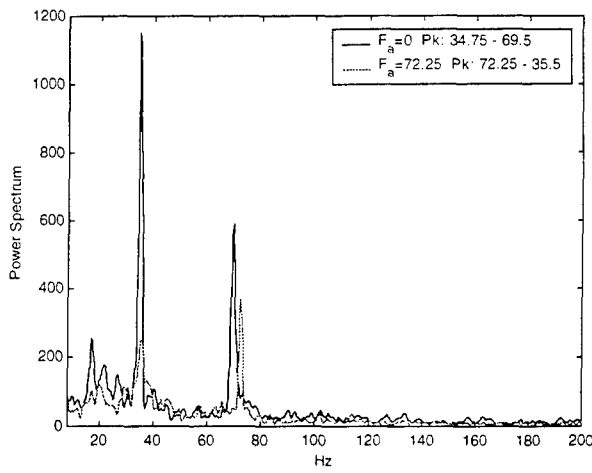
Fig. 12. PSD of pitot 3 at excitation |F|=2.06 . Angle of attack 30^\circ
