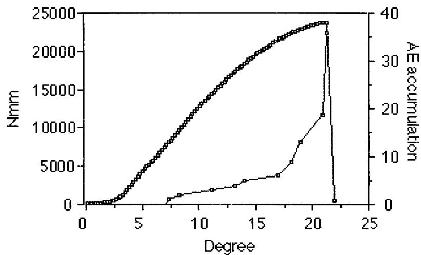
Fig. 3 Torque-torsional angle and AE accumulation-torsional angle curves.
