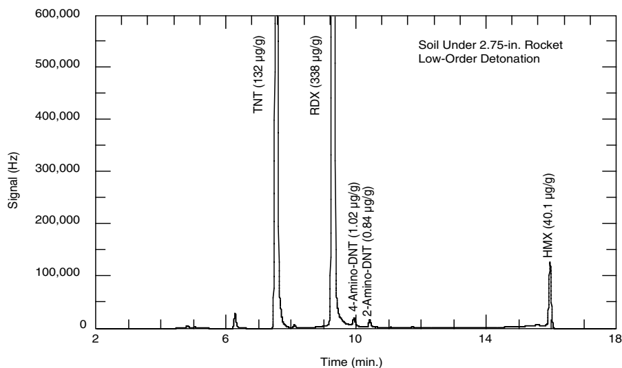
Figure 21. Chromatogram (GC-µECD) of solvent extract of soil collected under a 2.75-in. rocket warhead containing Composition B.
