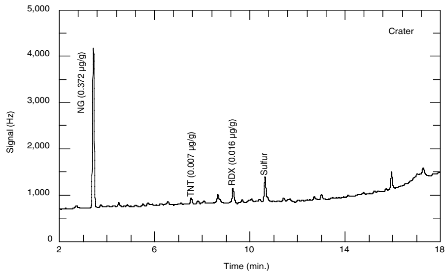
Figure 15. Chromatogram (GC-μECD) of solvent extract of soil collected 10 m from center of range maintenance crater.
