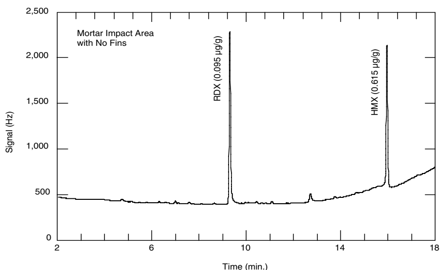
Figure 4. Chromatogram (GC- \mu ECD) from the extract of surface soil collected in an area with no mortar projectile fins. Low concentrations of RDX and HMX were found a short distance from the impact point.
