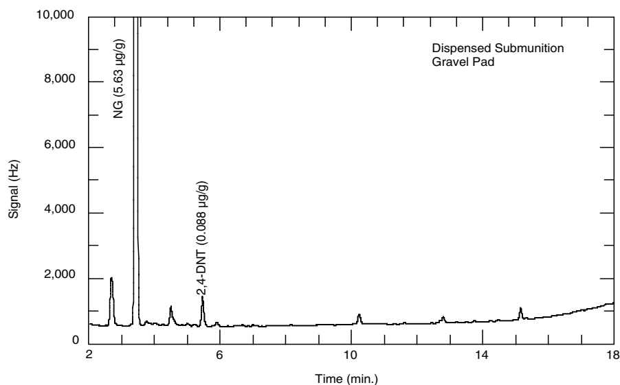
Figure 19. Chromatogram (GC-μECD) of solvent extract of soil collected on a gravel pad that had pieces of 2.75-in. low-spin folding fin aircraft rockets and grenades (M39 and M43A1) scattered over the surface.
