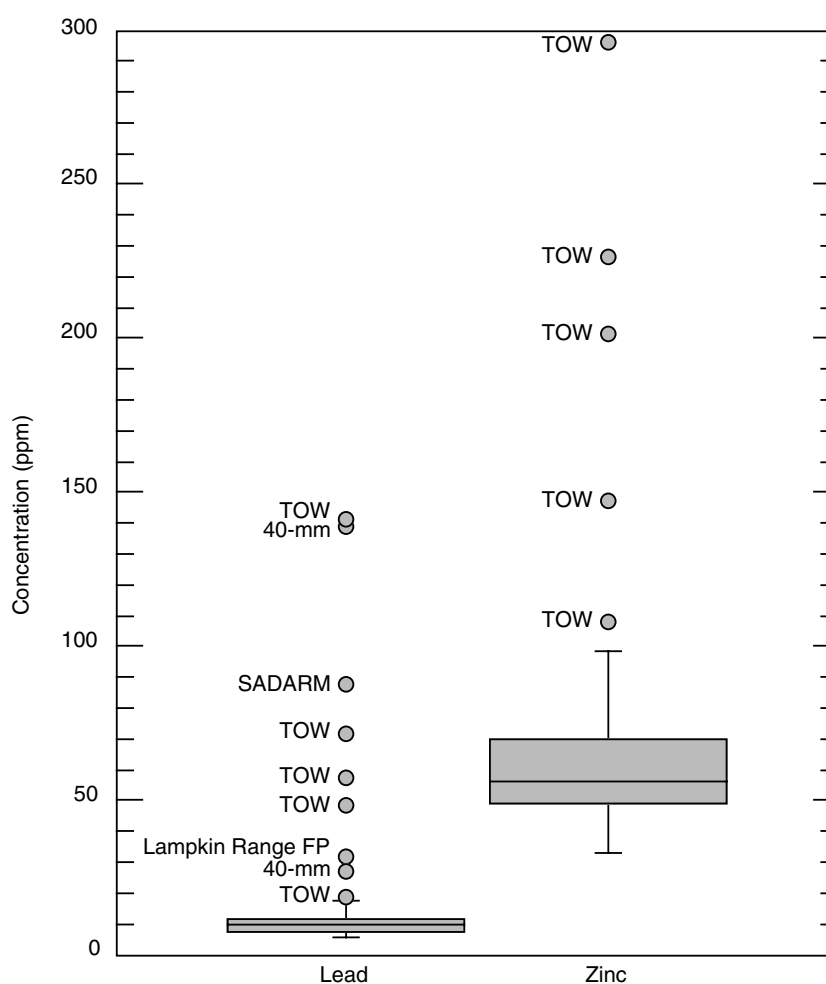
Figure 25. Box plots of lead and zinc concentrations showing which events resulted in increased metal concentrations. Each box encloses 50% of the data with the median value represented as a line in the box, the upper quartile as the top of the box and the lower quartile as the bottom of the box. The circles represent outliers, which are values greater than the sum of the upper quartile plus one and one-half times the difference between the upper and lower quartile.
