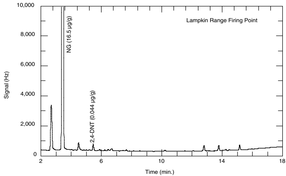
Figure 17. Chromatogram (GC-μECD) of solvent extract of soil collected at Lampkin Range firing point.
