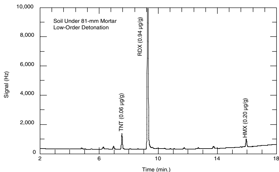
Figure 5. Chromatogram (GC-μECD) from the extract of surface soil collected under the low-order detonation of an 81-mm mortar projectile. The explosive composition was 66% RDX, 25% TNT, and 9% HMX, as determined by HPLC.
