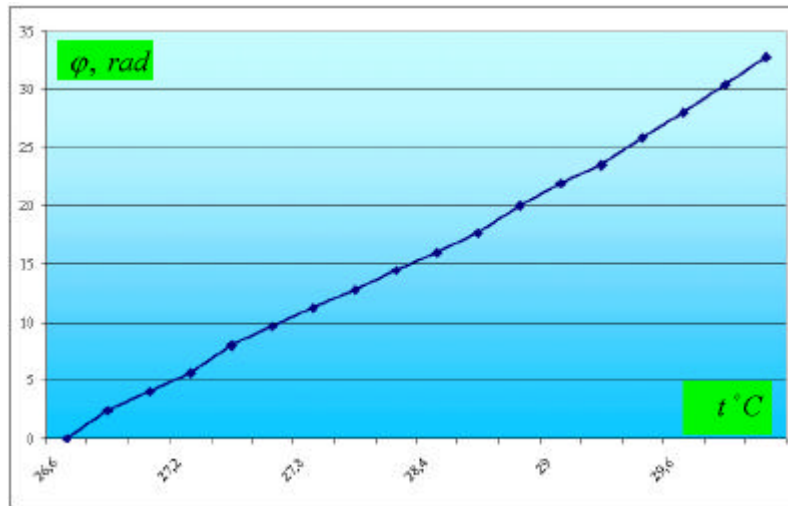
Fig.3. The experimental dependence of the rotation angle \varphi of the OV center on the temperature t °C. The experimental accuracy is about 1.5%, the fiber length is 30 m.
