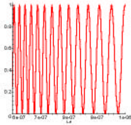
Fig.1. The spectral response S(l) of the optical fiber with IV vortex, \Delta\tilde{n}_0 \approx 10^{-9} , z=1 m.
