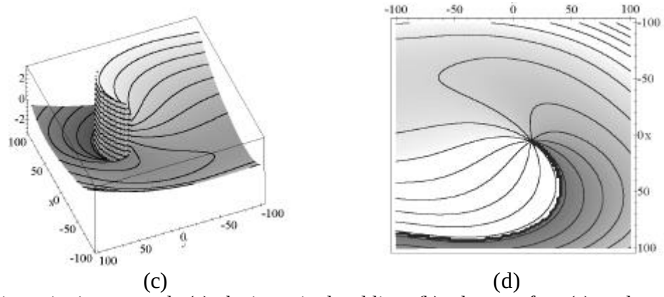
Fig.3. The intensity in gray scale (a), the intensity level lines (b), phase surface (c), and equal phase lines (d) for the optimal OV, calculated by eqs.(1) and (4) under z = 1000l , a = 0.08rad
