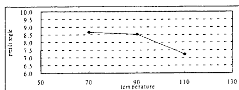
Figure 3. Temperature dependence of pretilt angle by The Taguchi method.
