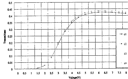
Fig. 10b Simulation results of the cell gap variations in FOP LCD
