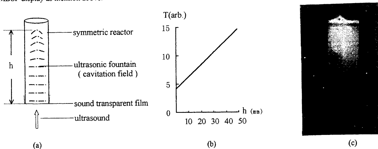
Fig.4 (a) ultrasonic fountain and its display set-up; (b) Rough temperature distribution along with the axis of the ultrasonic fountain ( h : height of the fountain; T : reading in one minute when the thermometer is set into the fountain); (c) MBSF picture of the ultrasonic fountain.
