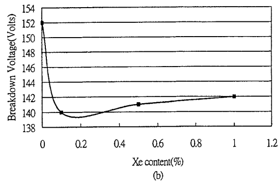
Fig. 7(b) The breakdown voltage with Xenon percentage.
