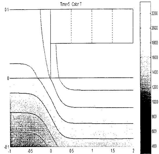
Fig. 2 Simulation of a temperature profile, in Kevine degree, at the edge of a recessed silicon film after laser irradiation. The upper region above zero is silicon and the bottom, silicon dioxide.
