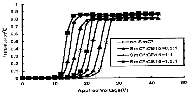
Fig. 2: Measured transmissions of the PSCT cells having y-times SmC* concentrations ( y = \text{SmC}^*/\text{CB15} ).
