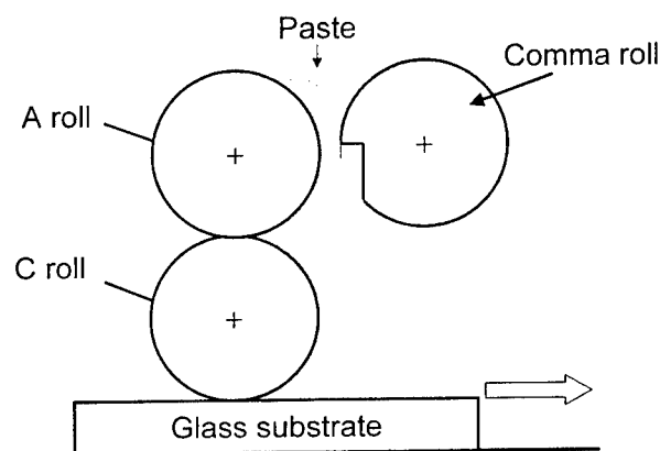
Figure 4. Roll Coating Method
