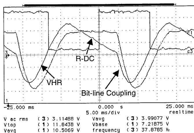
Figure 10 Flicker measurement of the SXGA light valve.
