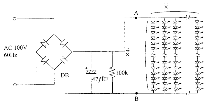
Fig. 2 A condenser-input type electric circuit
