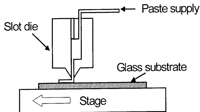
Figure 3. Slot Die Coating Method
