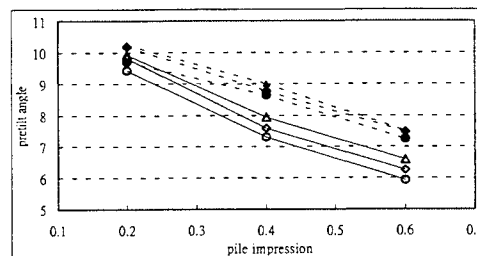
Figure 2. Effects of pretilt angle (measured data) with variable of each parameter.
