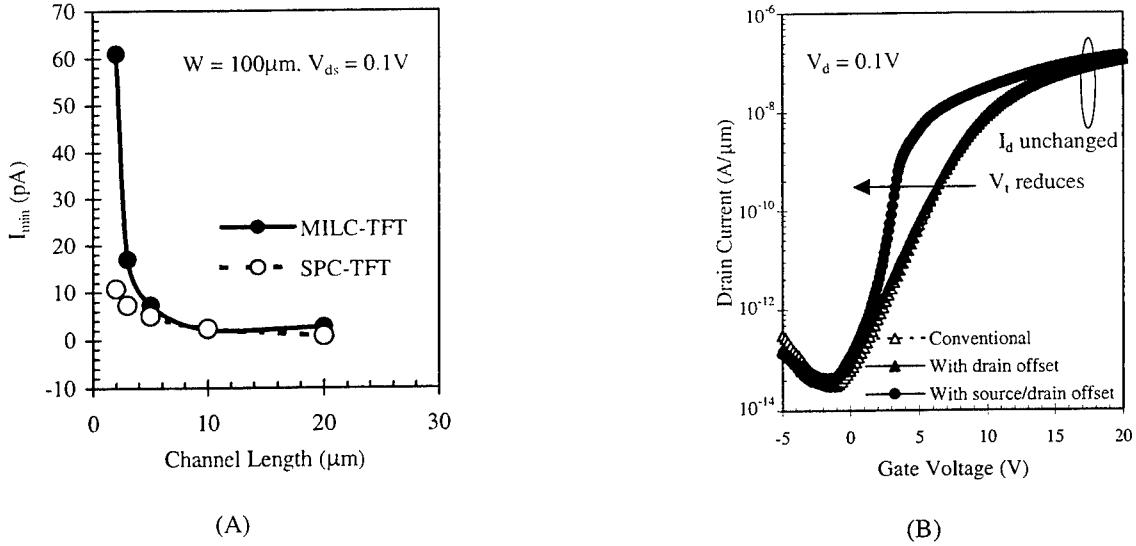
Figure 11. A) I_{min} vs L for N-channel “111”-MILC and SPC TFTs. B) I_d - V_g characteristics of the three different kinds of MILC TFTs: conventional, drain offset, and source/drain offset denote, respectively, “111”-, “110” and “010”-MILC TFTs.
