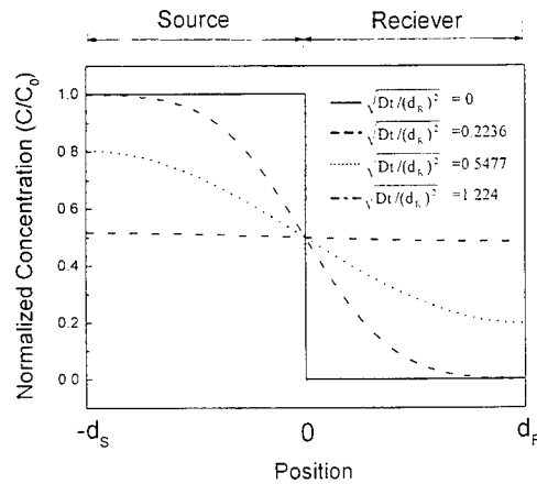
Fig. 2: Calculated normalized profiles of dye concentration C(x, t)/C_0 vs. normalized diffusion length \sqrt{Dt/dR^2} .
