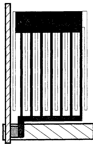
Fig. 2b FFS pixel structure
