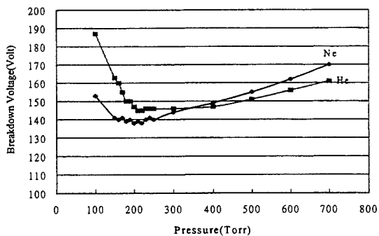
Fig. 8 The breakdown voltages for Helium and Neon at different gas pressure.
