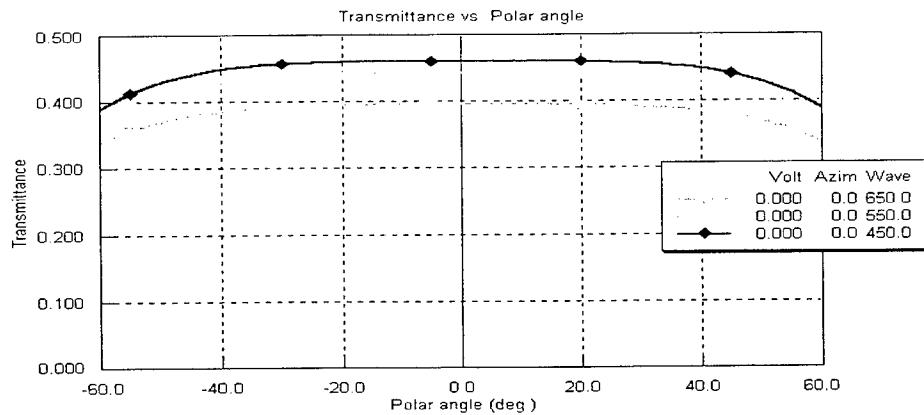
Figure 21. Special 0/90 two-domain TN/LCD Red/Green/Blue transmission vs. viewing angle, and gray scale levels No. 1 and 8, for horizontal viewing zone with A and C plates. LC: TL-203.
