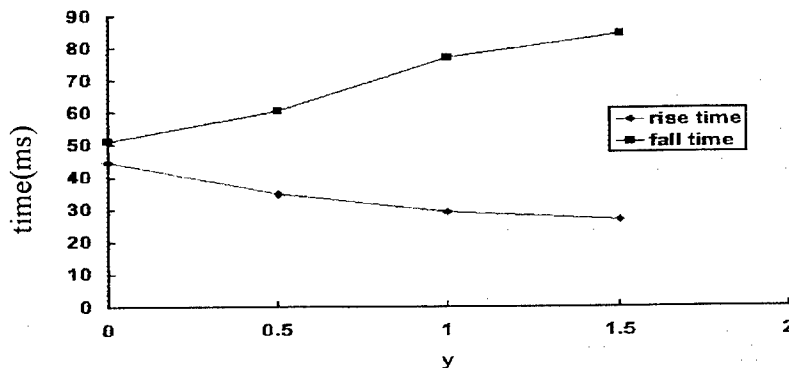
Fig. 3: The measured response times of the PSCT cells having y-times SmC* concentration ( y = \text{SmC}^*/\text{CB15} ).
