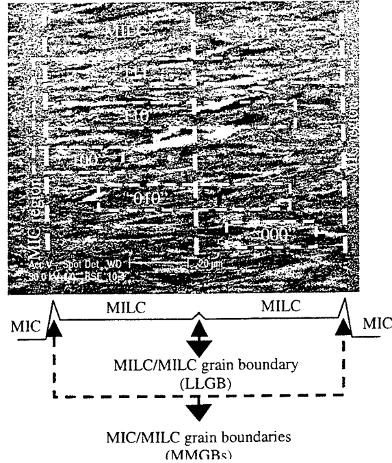
Figure 8. SEM micro-graph showing both MIC and MILC regions. A total of three GBs (two MMGBs and one LLGB) transverse to the MILC direction can be identified. The active areas of the five possible MILC TFTs are delineated by the five rectangular boxes superimposed on the micro-graph.
