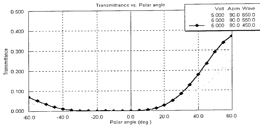
Figure 20. Normal 135/45 two-domain TN/LCD Red/Green/Blue transmission vs. viewing angle, and gray scale levels No. 1 and 8, for vertical viewing zone with not films. LC: TL-203. 20(a)
