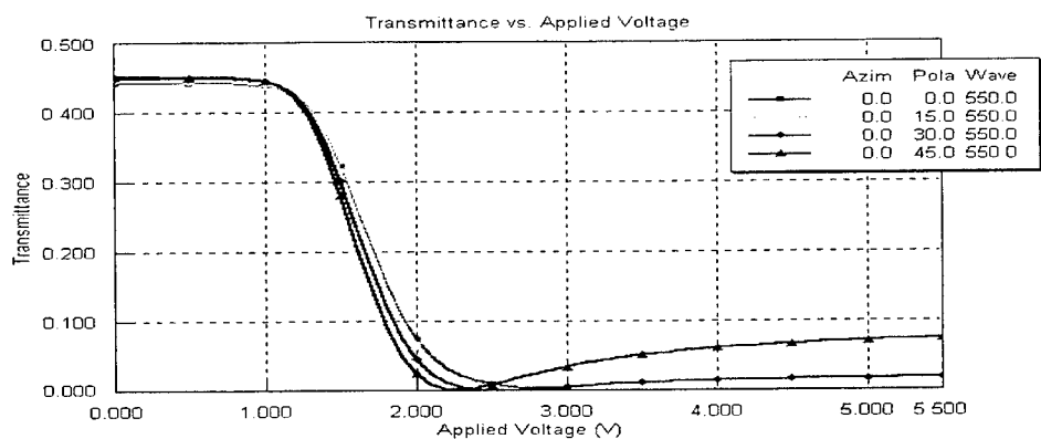
Figure 1. Standard one-domain and two-domain TN/LCD transmission vs. voltage for normal incident, \pm 15^\circ , \pm 30^\circ , and \pm 45^\circ in the horizontal viewing zone. LC: TL-203.
