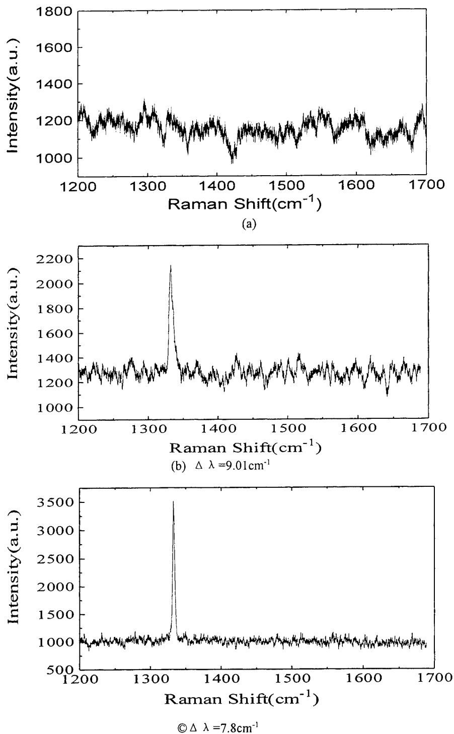
Fig.3 Raman spectra of different samples
