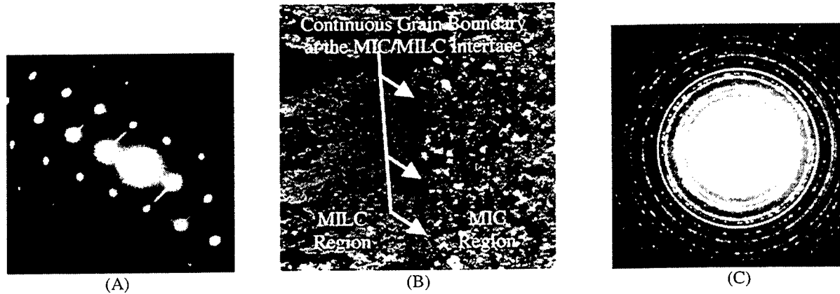
Figure 6. A) TED micro-graph in the MILC area, showing predominantly \{110\} orientation, B) TEM micro-graph showing elongated grains in the MILC region. A distinct grain boundary (MMGB) separates the MIC and the MILC regions, and C) TED micro-graph in the MIC area.
