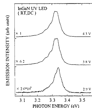
Fig.2 (a) Emission spectra obtained at RT between 2.9 and 4.1 V.
