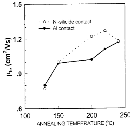
Figure 5. Changes in the field effect mobility of the a-Si:H TFTs with Ni-silicide and Al S/D contacts. W/L = 12 \mu m/6 \mu m.
