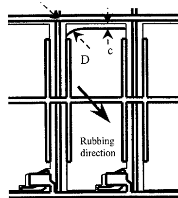
Figure 2.2 Structure of 6.4" pixel
