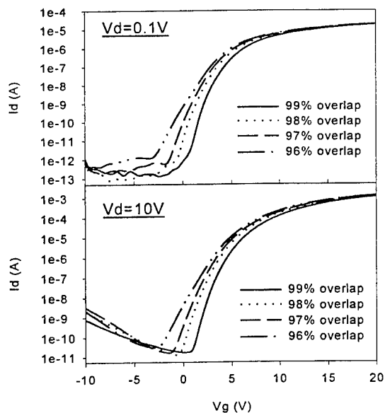
Figure 9 The typical I_d - V_g curves ( V_d=0.1 and 10 volt) of n-type single-gate TFT ( W/L = 50/20\mu m ) with various laser overlapping ratios (96%~99%).
