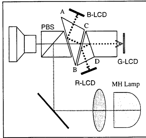
Figure 6 Layout of the compact optical projector with one PTA and one PBS.
