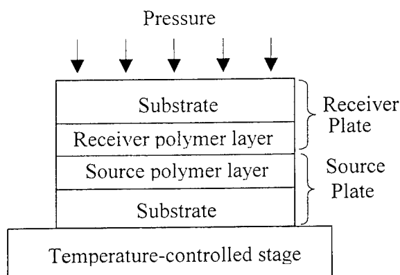
Fig.1. Arrangement for finite-source dye-diffusion thermal transfer.
