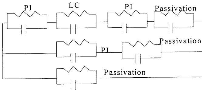
Fig. 11c The equivalent circuit of FOP.
