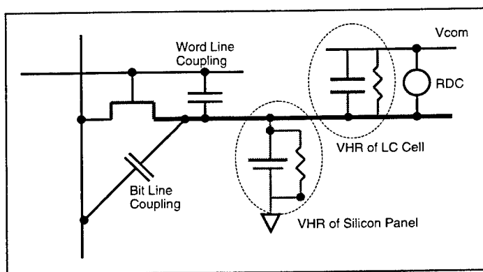
Figure 8 Flicker model of the pixel in silicon light valve.
