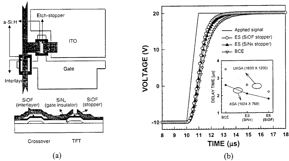
Figure 9. The plan and cross-sectional views of the pixel structure of a TFT-LCD for the application of a SiOF etch stopper (a), and the charging behavior of a pixel during gate pulse and the delay signal waveform for the three-different structures (b). A resolution of UXGA was used.
