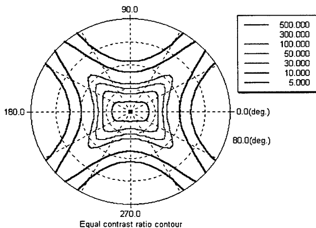
Figure 9. Standard two-domain TN/LCD CR contour plot at 5.0 volt. LC: TL-203.
