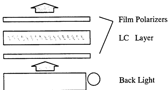
Fig. 3 Optical Components of LCDs
