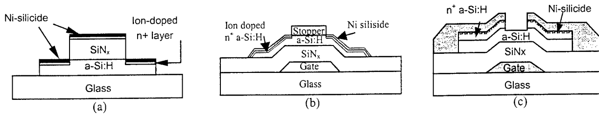
Figure 4. Cross-sectional views of the fabricated TFTs: coplanar a-Si:H (a), ES a-Si:H(b), BCE a-Si:H (c).
