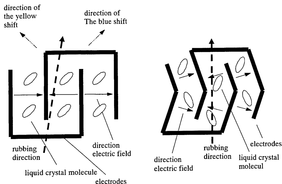
Fig. 10 Inter Digital Electrode Structures for IPS and S-IPS
