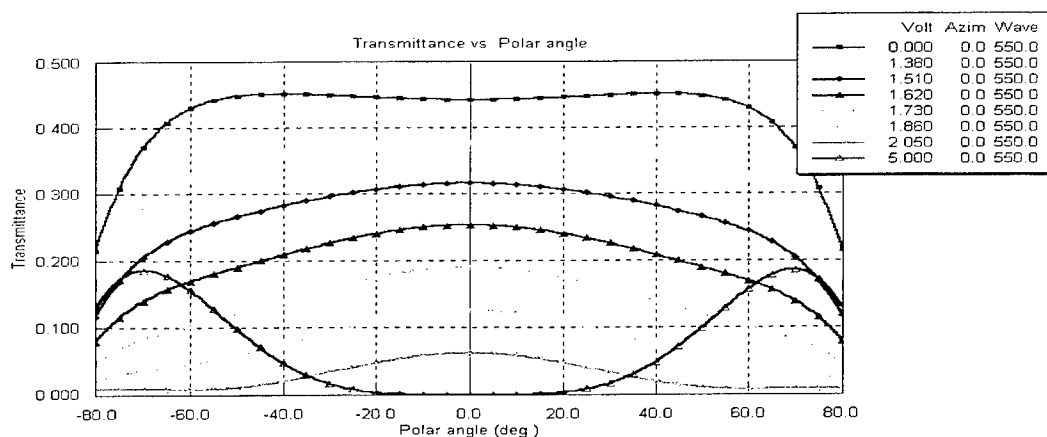
Figure 5. Standard one-domain TN/LCD transmission vs. viewing angle and gray scale level for vertical viewing zone. LC: TL-203.
