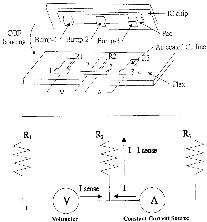
Figure 9. Schematic illustration of the R_2 contact resistance measurement by using the 4 points test method and its corresponding circuitry.
