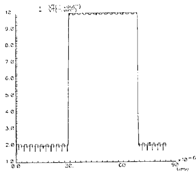
Figure 3.6 (a) the step response of the circuit in UMC model
