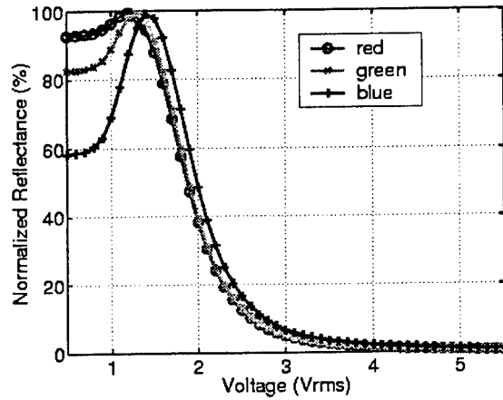
Figure 4 The characterized reflectance-vs-voltage curves of the MTB LC cell on the SXGA silicon panel.
