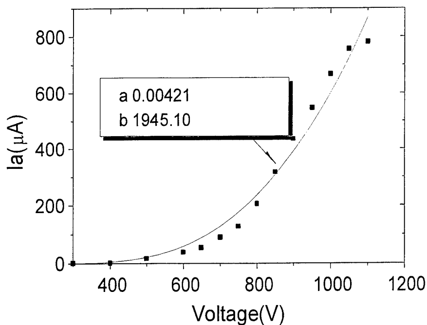
Fig.4(b) field emission performance of complex diamond conduct ceramic thin film after acid treatment
