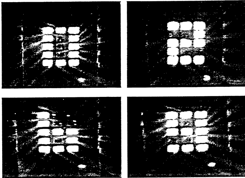
Fig. 4 Electron emission image of 15-pixels CNTs-emitter using diode structure, operated at 5 V/ \mu\text{m} applied electric field.
