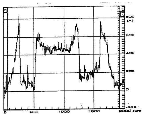
Figure 4 The surface topography of single pulse excimer laser crystallized poly-Si film.
