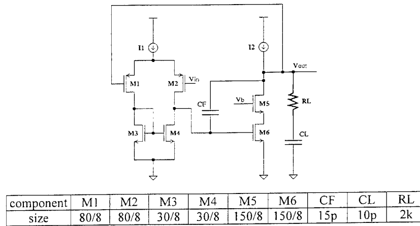
Figure 3.3 the operational amplifier schematic and the size
