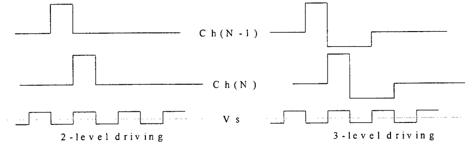
Fig. 9 The driving wave-form of the Scan bus
