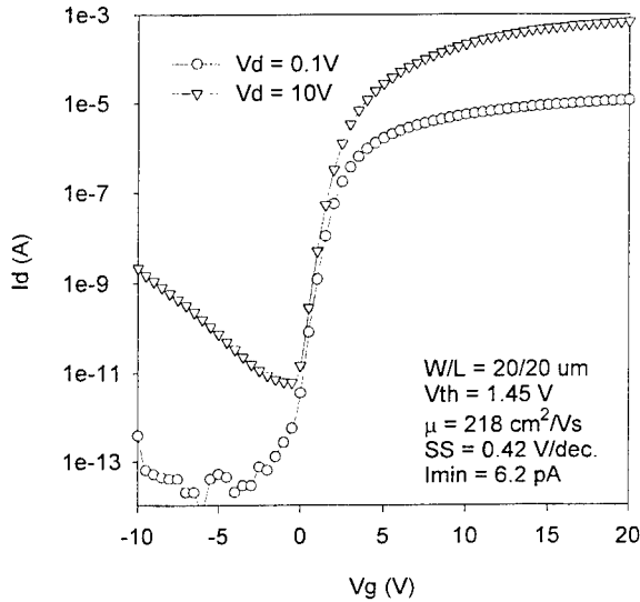
Figure 1. Typical TFT Id-Vg curves.
