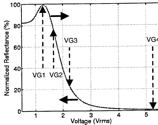
Figure 5 Fine tune of the green curve of the MTB cell through four gamma correction voltages.
