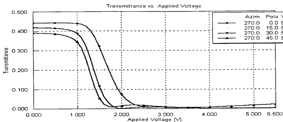
Figure 3. Standard one-domain TN/LCD transmission vs. voltage for normal incident, -15^\circ , -30^\circ , and -45^\circ in the vertical viewing zone. LC: TL-203.
