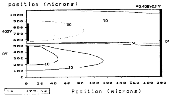
Electric potential : Ne-4%Xe, 500Tor
