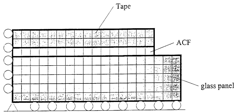
Fig. 3 Finite element model of connector
