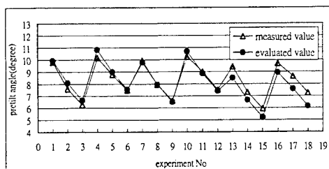
Figure 1. The deviations between measured data and evaluated data by The Taguchi method.
