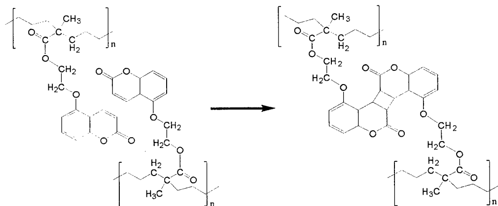
Fig.1 The structure of two actinic copolymers (left) and their dimerization (right) by intermolecular photo-induced (2+2) cycloaddition
