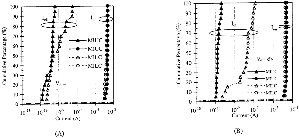
Figure 15. Statistical distributions of I_{on} and I_{off} for (A) n-type and (B) p-type MIUC ("000"-MILC) and "111"-MILC TFTs with W/L = 10/5\mu m.
