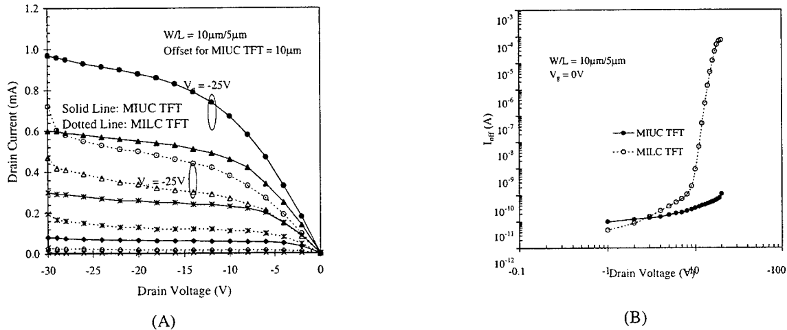
Figure 14. A) I_d dependence on V_{ds} from V_g = -5V to -25V at -5V interval for p-channel MIUC (solid lines) and “111”-MILC (dotted lines) TFTs. Earlier drain breakdown can be clearly observed in the conventional MILC TFTs. B) Leakage current ( I_{off} ) dependence on V_{ds} .
