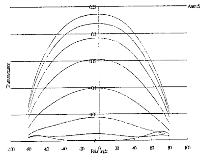
Fig. 8b 8 gray levels of FOP
