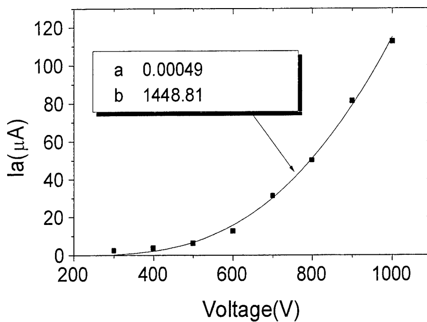
Fig.4(c) Field emission performance of diamond grains deposited on silicon by electrolyte
