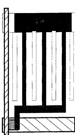
Fig. 2a IPS pixel structure
