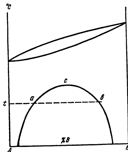
Fig. 152. Diagram of Phase Transitions with Decomposition of Solid Solutions.
