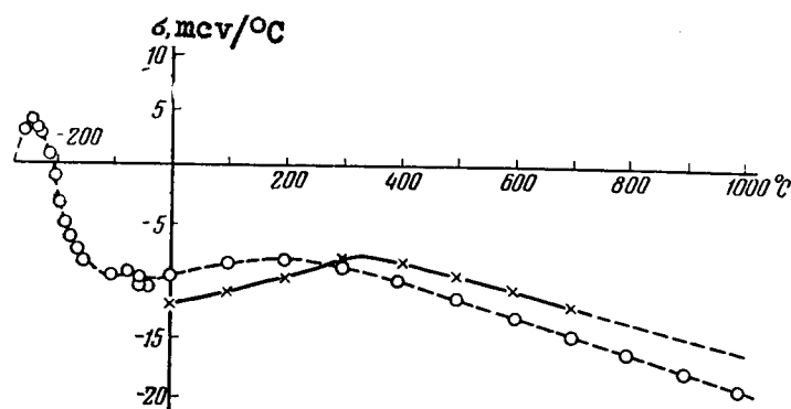
Fig. 49. Thomson emf of Spectrally-Pure Platinum:
